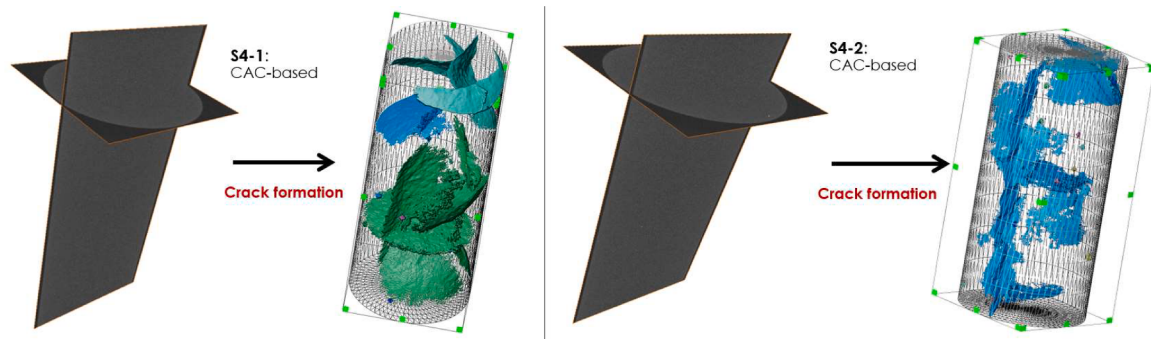
Fig. 6. Microstructure of samples S4-1(left) and S4-2 (right) before and after quenching. Voxel resolution of 32\ \mu\text{m} . Samples are of sealant composition S4, CAC-based. Connected cracks and occasional new voids develop in both samples.
