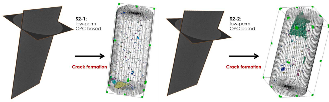
Fig. 4. Microstructure of samples S2-1(left) and S2-2 (right) before and after quenching. Voxel resolution of 32\ \mu\text{m} . Samples are of sealant composition S2, low-permeability OPC-based. Some connected cracks and visible new voids develop in both samples.
