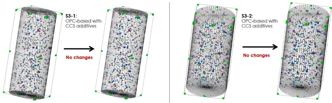
Fig. 5. Microstructure of samples S3-1(left) and S3-2 (right) before and after quenching. Voxel resolution of 32\ \mu\text{m} . Samples are of sealant composition S3, OPC-based with CCS additives. There are no obvious changes after quenching in either sample.
