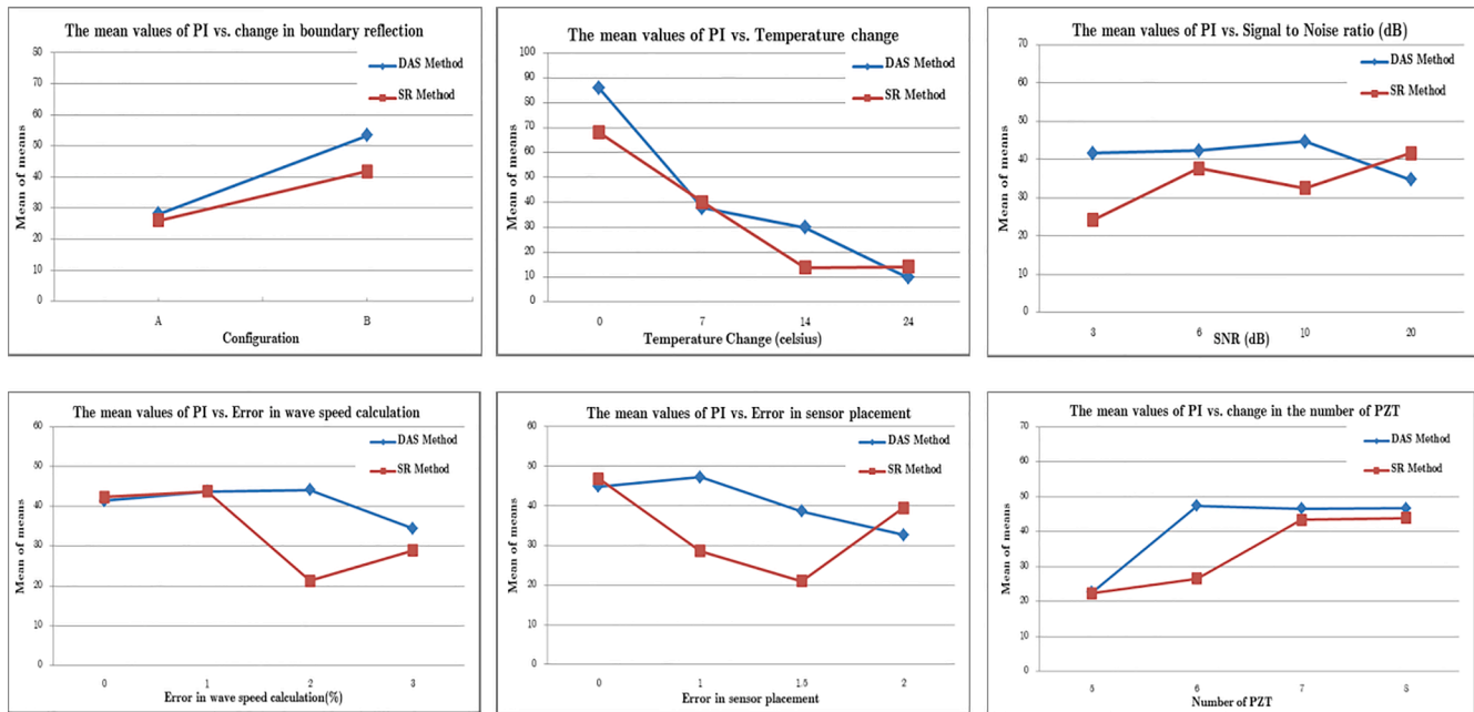
Fig. 12. Main effect plot for means for results of the DAS and SR methods.
