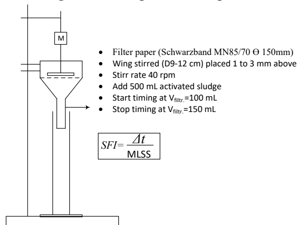
Figure 4 Sludge filtration Index (SFI) to determine filterability. Adapted from (Geilvoet, 2010)
