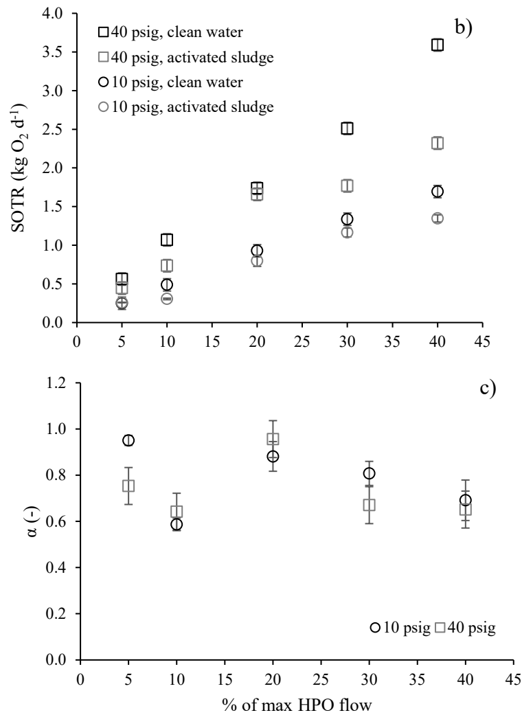
Figure 49 Influence of pressure and suspended solids on the process parameters in clean water and mixed liquor. (a) Mass transfer coefficient k_{La} (h -1 ), (b) SOTR (kg O 2 d -1 ), (c) alpha factor (-)
