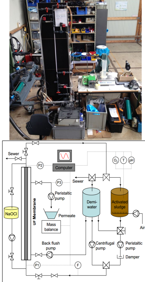
Figure 5 The Delft Filtration Characterization installation (DFCi) (Maria Lousada-Ferreira et al., 2014)
