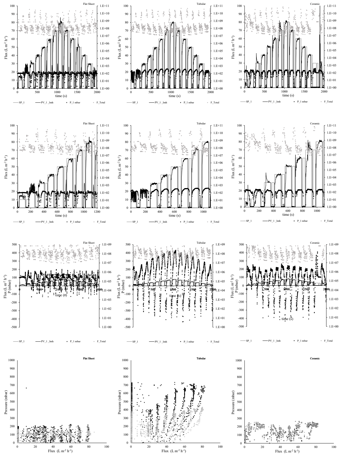
Figure 60 Membrane filtration characterization at 20 \text{ g L}^{-1} . Column 1: Flat sheet, column 2: Tubular, column 3: Ceramic
