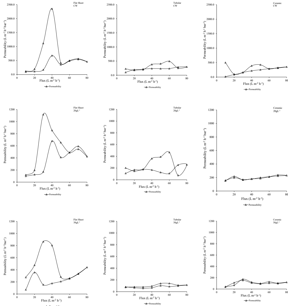
Figure 62 Pressure profiles, Permeability for three submerged membranes in clean water (CW) and activated sludge with MLSS 20 and 38 \text{g L}^{-1} .
