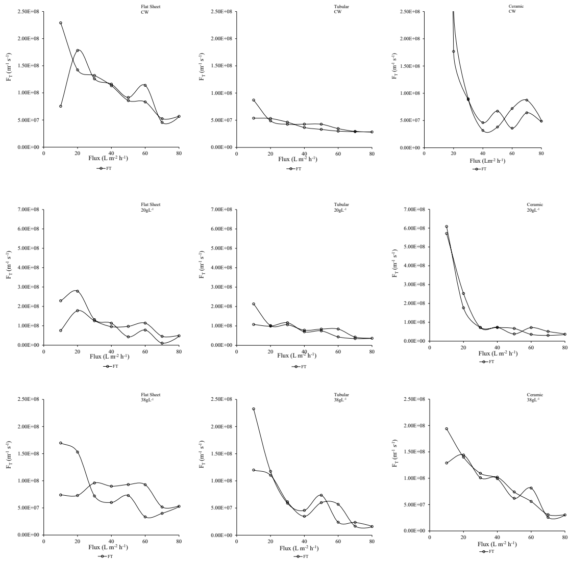
Figure 63 Total fouling rate for three submerged membranes in clean water (CW) and activated sludge with MLSS 20 and 38 \text{g L}^{-1} .
