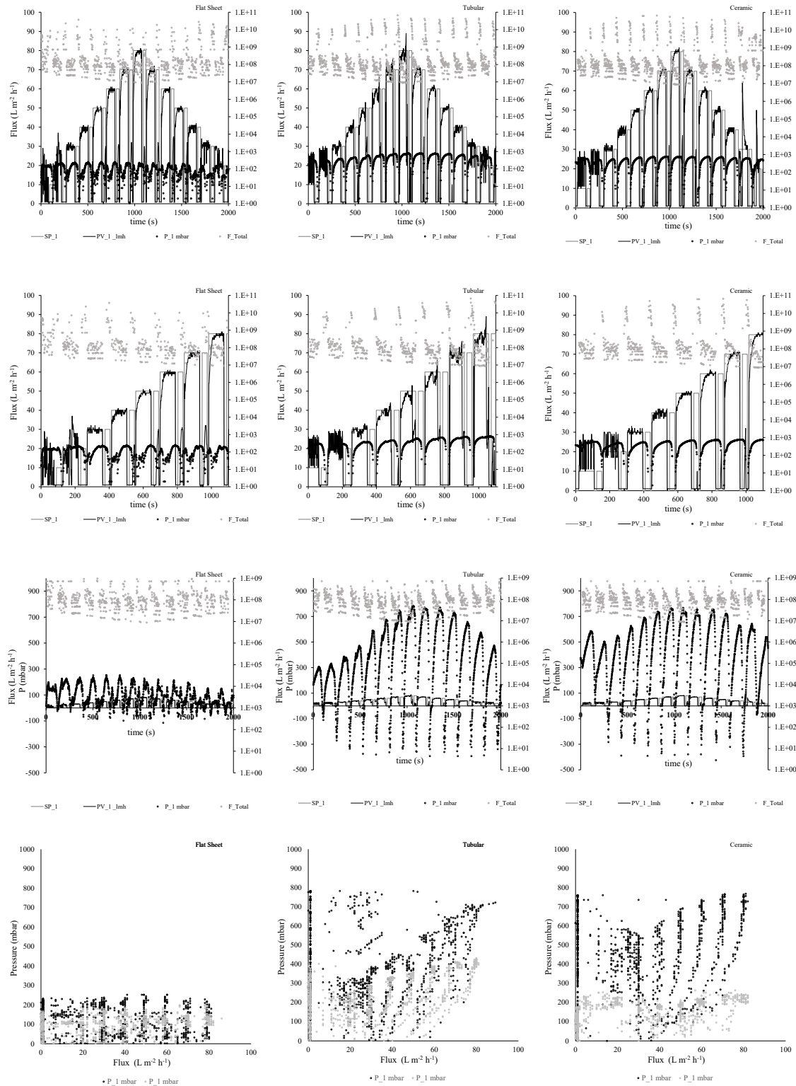
Figure 61 Membrane filtration characterization at 38 \text{ g L}^{-1} . Column 1: Flat sheet, column 2: Tubular, column 3: Ceramic
