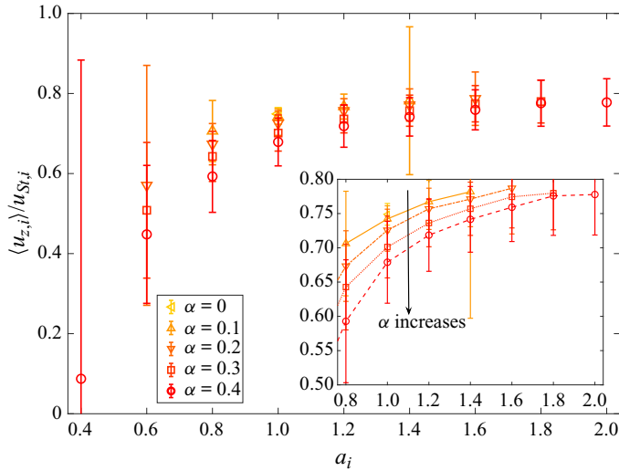
Figure 12. Normalised average settling velocity of each size class for different polydispersity parameters and \phi = 0.05 . The inset is a zoom in the range 0.8 \leq a_i \leq 2.0 . The lines are guides for the eye.
