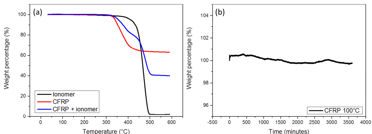
Figure S 1 TGA temperature ramp of the individual components of the CFRP-ionomer composite (a) and the residual weight of the CFRP during an isothermal treatment of 100°C.
