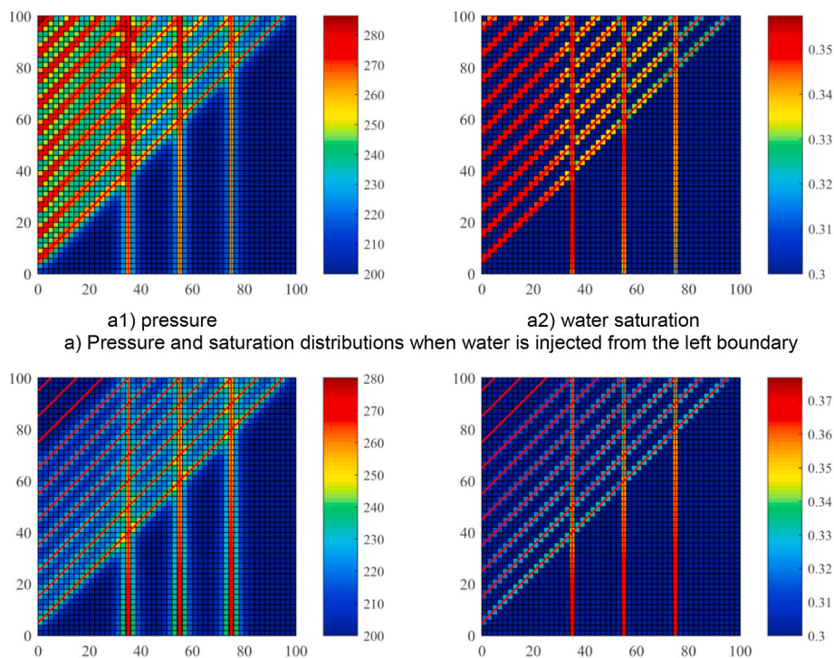
Fig. 3. The effect of flow direction on the flow response in a local fractured domain. We inject water at the left or bottom side of the fracture network with constant bottom hole pressure. a) Pressure and saturation distributions when water is injected from the left boundary, b) Pressure and saturation distributions when water is injected from the bottom boundary.
