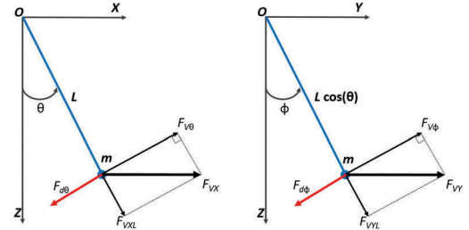
(a) Forces on the XZ plane.
