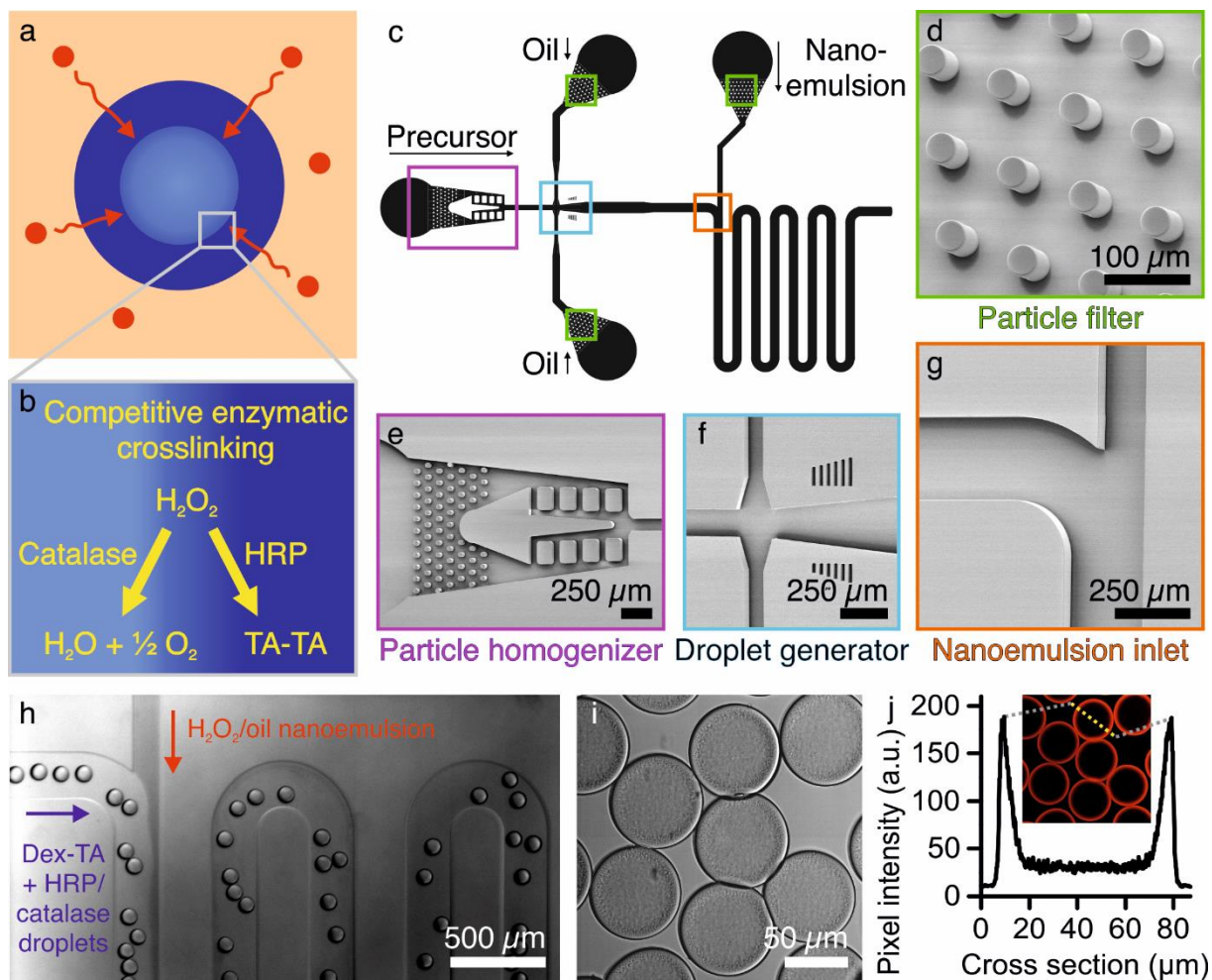
Figure 4. Hollow microcapsules production using nanoemulsion-induced enzymatic crosslinking.
