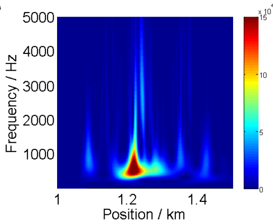
(c) measurement 1 trailing axle
