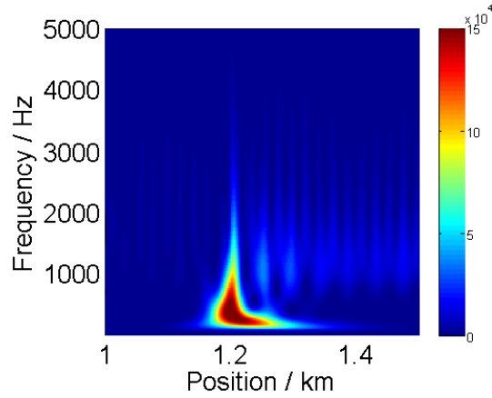
(a) simulation result
