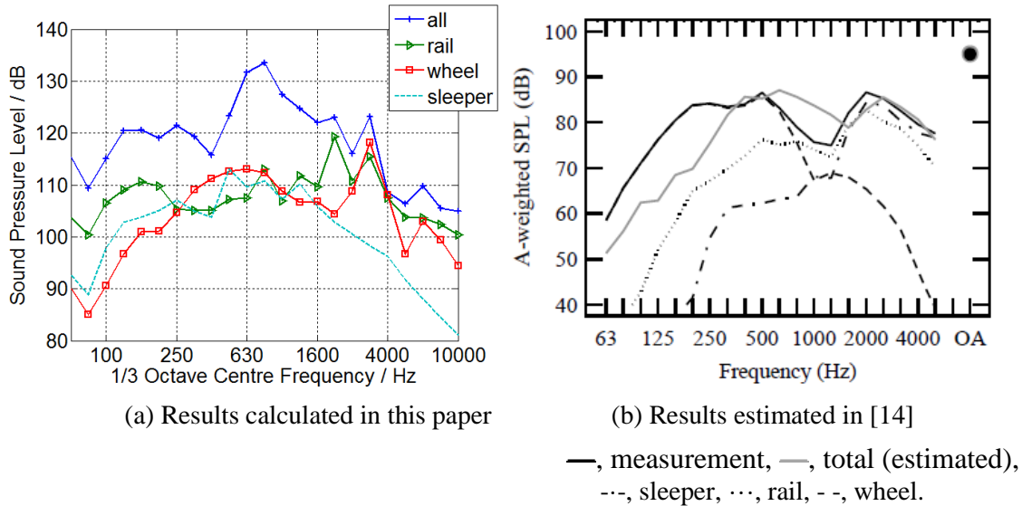
Figure 10: Noise contribution
