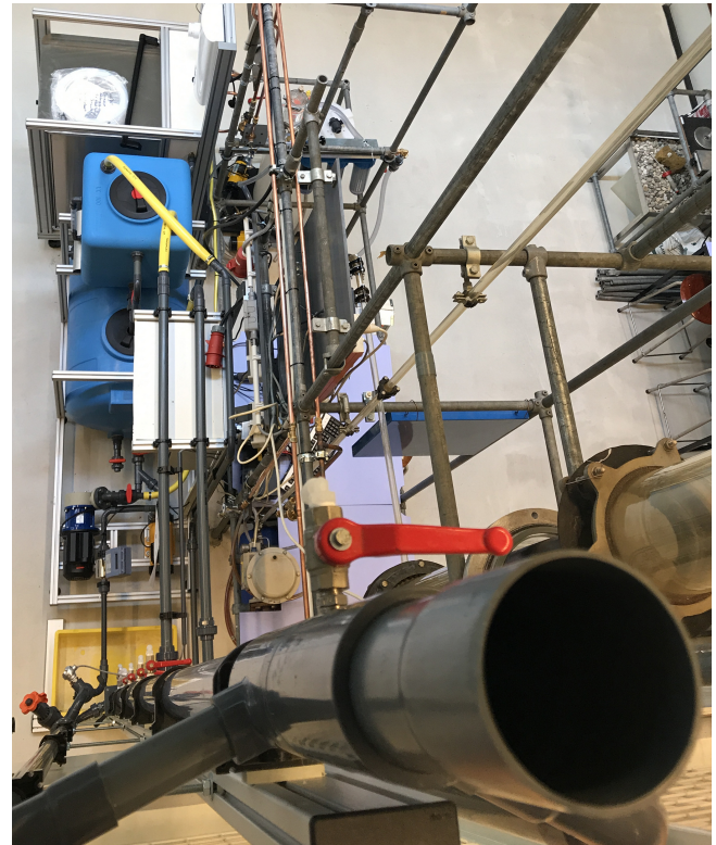
Figure 1. Experimental pilot set-up in Amsterdam, Utrecht, and London. D = 57 mm, with temperature control column (top view).
