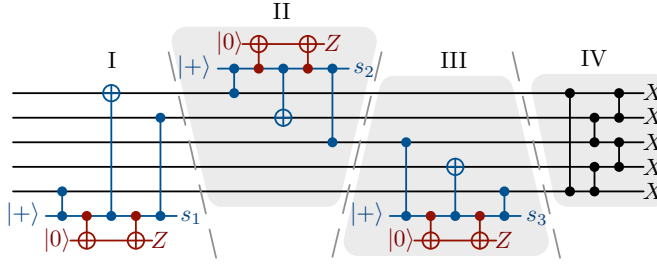
Figure 4.2: Circuit used to measure the logical X operator X_1 X_2 X_3 X_4 X_5 on a logical qubit of the 5-qubit code. The circuit is divided into four labeled portions. Depending on the results of previous measurements, the last three portions may be skipped. The stabilizer measured here s_1, s_2, s_3 (lowercase) are all weight-3 logical X operators of the 5-qubit code. Additionally, the circuit includes an extra ancilla qubit in red known as the flag qubit, which is crucial for ensuring fault-tolerance. Figure taken from Ref. [9]
