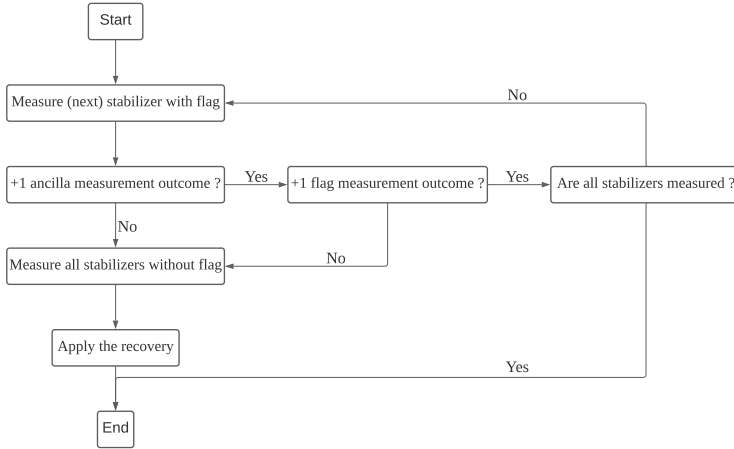
Figure 4.4: The flowchart of a full flag error correction cycle proposed by Chao and Reichardt [9]. For the 5-qubit code, the stabilizers are s_1 = XXYYIY , s_2 = YXXYI , s_3 = IYXXY and s_4 = YIYXX . The stabilizer measurements without flag give a 4-bit error syndrome, which determines the recovery operation. Note that the error syndrome is interpreted differently depending on whether there is a raised flag. In the experiments presented in this work, we apply one stabilizer measurement of this error correction cycle and characterize the resulting post-measurement state.
