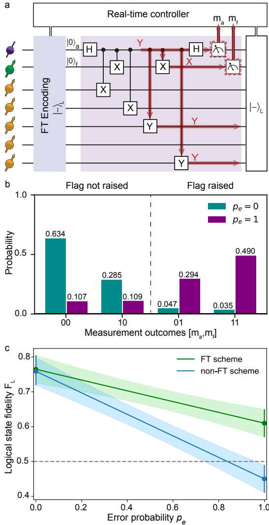
Figure 5.5: Fault-tolerant stabilizer measurement. a) Circuit diagram to measure the stabilizer XXYY on the encoded state. As an example to illustrate the compatibility with fault-tolerance we insert a Y error on the auxiliary qubit. This error will propagate to the 2-qubit error Y_3 Y_5 on the data qubits, which leads to a logical Z error. However, because the error also triggers the flag qubit it can be accounted for (Methods). b) Probability of the measurement outcomes of the auxiliary qubit ( m_a ) and flag ( m_f ) qubits when inserting ( p_e = 1 ) or not inserting ( p_e = 0 ) the Y error on the auxiliary qubit. The results show that the flag qubit successfully detects this error. c) Logical state fidelity F_L after the stabilizer measurement as function of the error probability p_e . The non-FT case does not take the flag outcome into account. Values between p_e = 0 and p_e = 1 are calculated as weighted sums (Methods).
