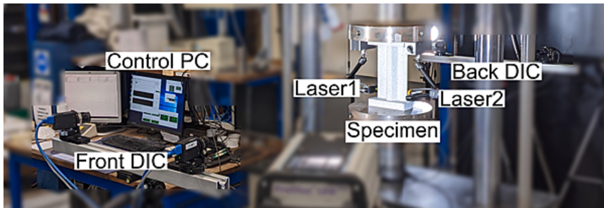
Fig. 5. Experimental Setup at Delft University of Technology.
