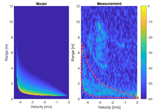
Fig. 5. Comparison of predicted (left) and measured (right) normalised range-Doppler signatures in decibels of an asphalt road surface when the car is moving at a speed v_c of 15 km/h.
