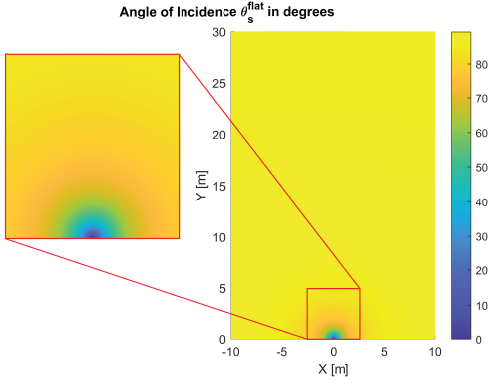
Fig. 2. Angle of incidence \theta_s^{flat} for a surface without undulations for a radar mounting height h_r of 50 cm.
