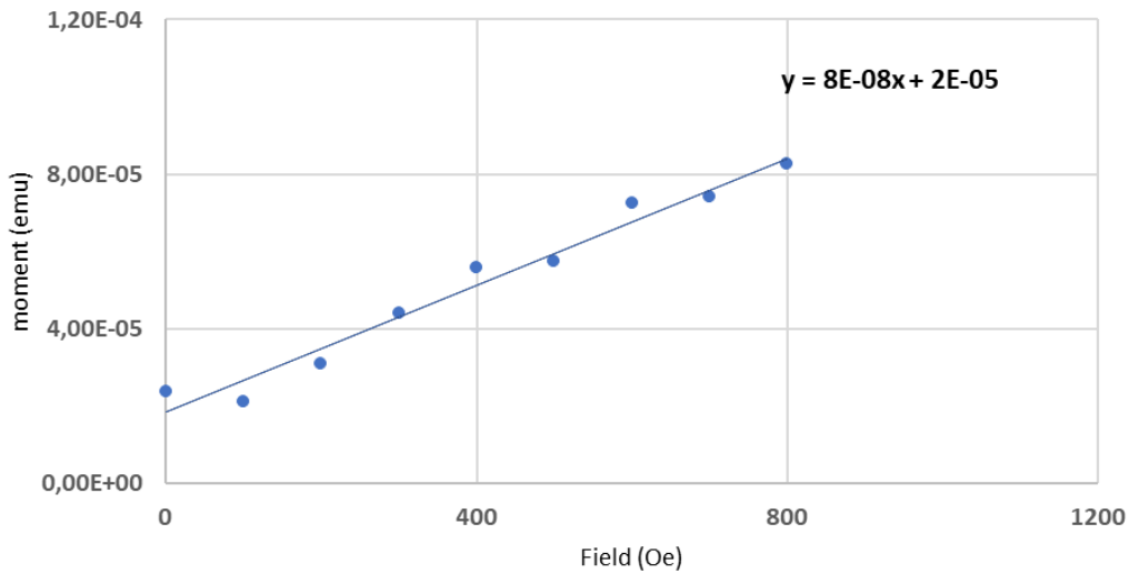
Figure S3-10: SQUID measurement of Fe 3+ quick addition pH 3 precipitate
