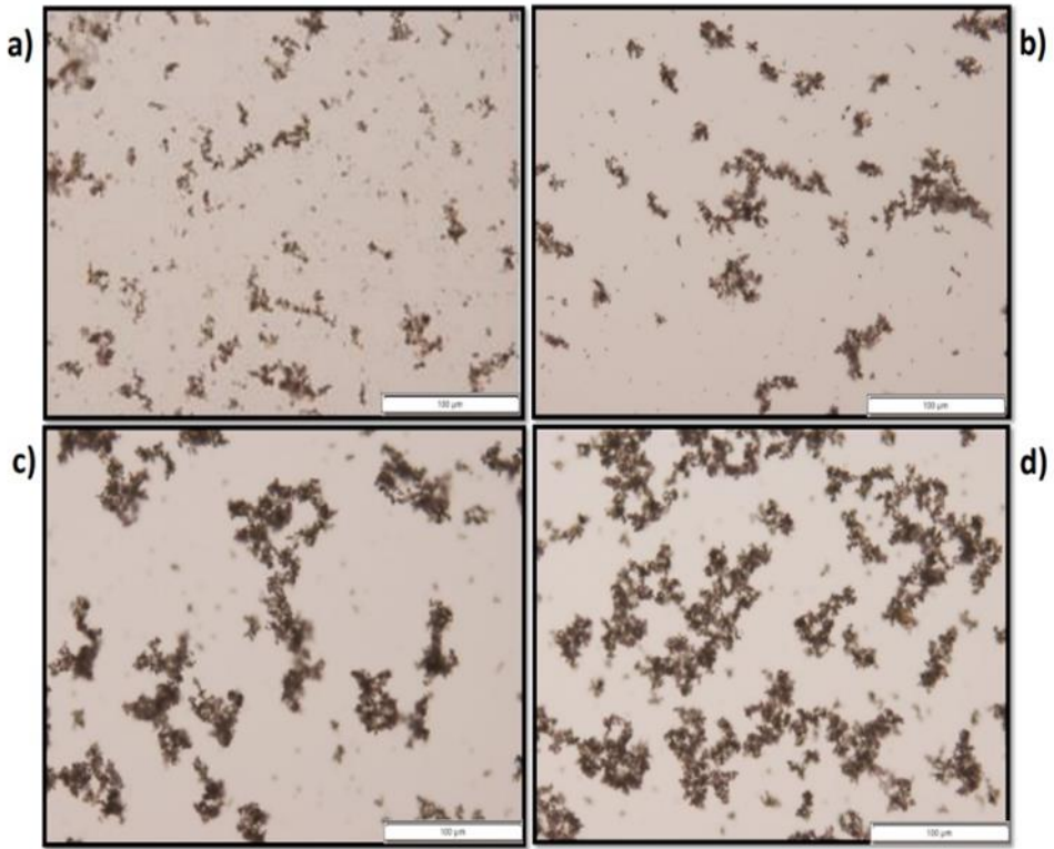
Figure 3-1: Fe (III)-P precipitation growth dosing Fe (II) over time under air oxidation conditions pO 2 = 0.2 bar a) 2 days, b) 4 days, c) 6 days, d) 10 days under the optical microscope. Scale =100μm
