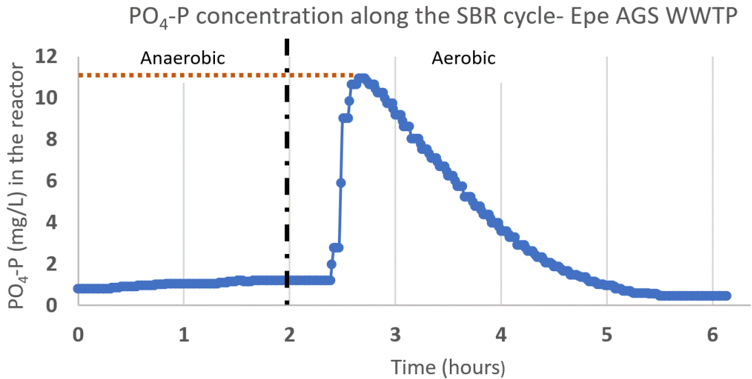
Figure 6-3: Online measurement data of PO 4 -P concentration in an AGS reactor in Epe WWTP from the sampling campaign work performed in Chapter (2)
