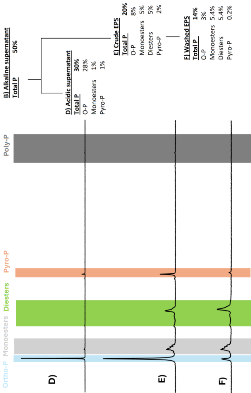
Figure 4-5: 31 P NMR spectra of the second step of the EPS extraction process: D) acidic supernatant, E) crude EPS, F) washed EPS- Epe municipal WWTP- All % are related to the initial total P in initial sludge approximated to the first whole numbers or first decimal point
