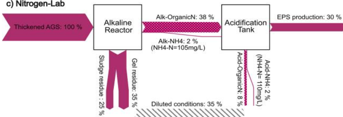
Figure 2-3: Mass balanced for laboratory scale undiluted extractions performed on AGS samples from Epe WWTP. Results are average from triplicates measurements. All percentages express % of the original sludge sample. The shaded grey arrow shows the amount of C, P, or N going to the acidic stream in the case of the diluted protocol. a) TCOD (organic solids), b) The dotted orange arrow shows the amount of bound phosphorus, and the shaded orange arrow shows the amount of free ortho-phosphate, c) The dotted arrow shows the amount of organic nitrogen
