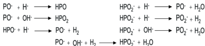
C) Radical chain reaction of P-based FRs in the gas phase
