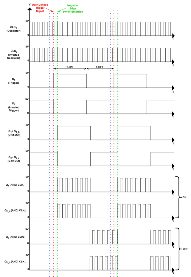
FIGURE 12. Detailed timing diagram for circuit, as presented in Fig. 14, where user-defined ON and OFF trigger signals are modulated over 167 kHz complementary digital signals to drive the coil between the full-bridge circuits.
