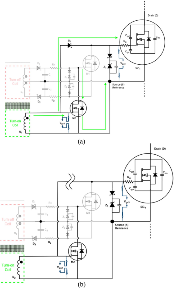
FIGURE 13. Illustration of the turn-ON mechanism for series-connected SiC MOSFETs, highlighting M_2 's role in synchronizing with SiC 1 and controlling M_1 , with D_3 charging C_{iss} to switch SiC 1 ON, and timing diagram correlation with Fig. 15. (a) Circuit during positive half voltage pulse. (b) Circuit during negative half voltage cycle.
