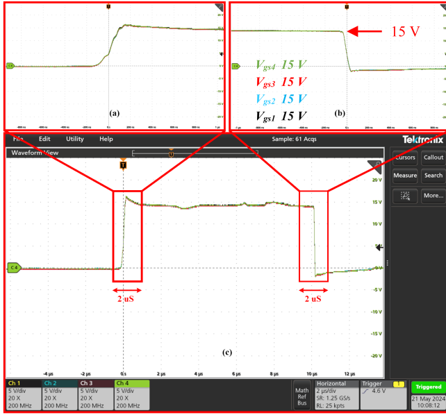
FIGURE 27. Gate-to-source ( V_{gs} ) voltage across four SiC MOSFETs in series during turn-ON and turn-OFF.
