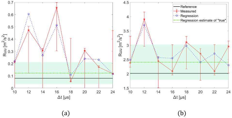
Figure 5.11. Reference, measured and regression Reynolds stresses with the estimates of "true" Reynolds stress ( \hat{R}_{uu,true} ) at (a) a point [(x/c, y/c) = (0.23, 0.17)] in the potential flow region I and (b) a point [(x/c, y/c) = (0.23, 0.07)] in the turbulent region II, the two regions being marked by rectangles in figure 5.5(b). Red error bars and green shaded regions represent one standard deviation uncertainty in the measured and estimated "true" Reynolds stress, respectively
