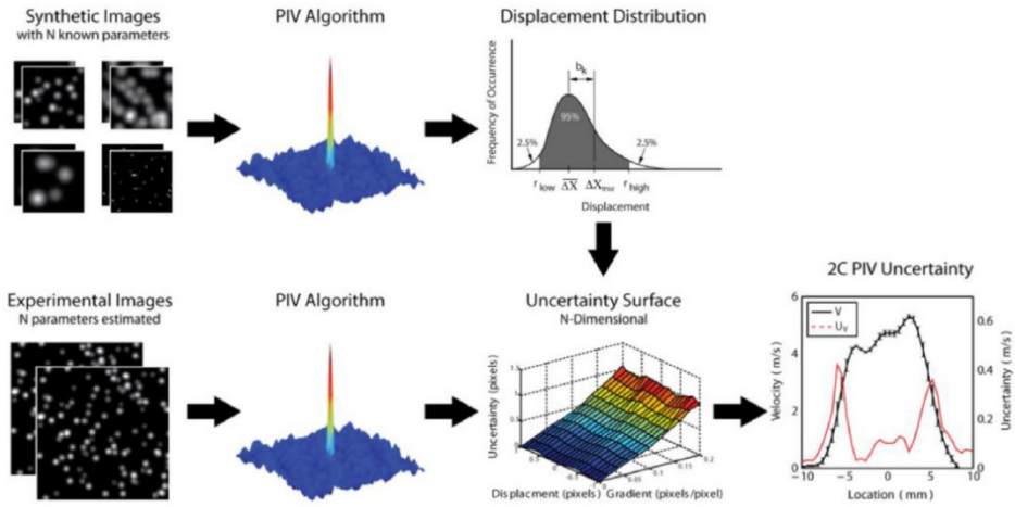
Figure 3.6. Schematic representation of the working principle of the uncertainty surface method (Siacchitano 2019)
