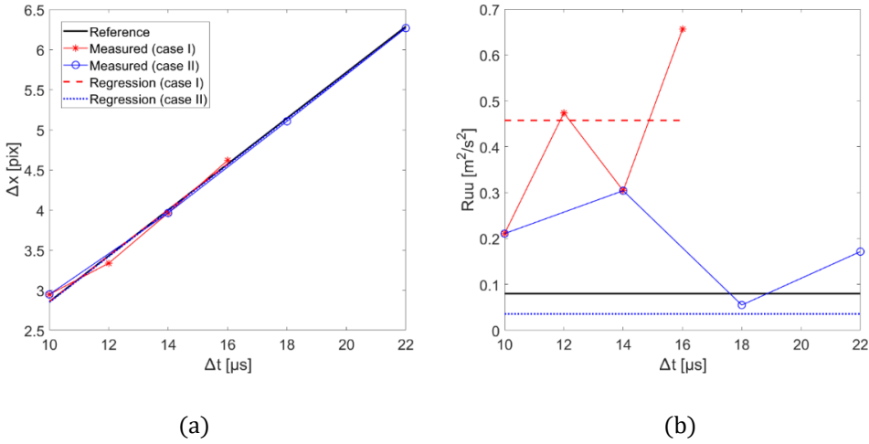
Figure 5.14. Measured and corrected (a) displacements and (b) Reynolds stresses at a point [(x/c, y/c) = (0.23, 0.17)] (case I: \Delta t 's = 10, 12, 14, 16 μs and case II: \Delta t 's = 10, 14, 18, 22 μs)
