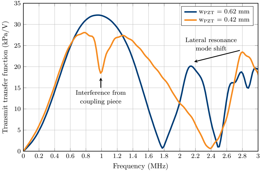
Figure 4.7: Transmit transfer functions obtained from Finite Element simulations of a 37-element HK1HD PZT transducer array with h_{\text{PZT}} = 0.35\lambda_{\text{PZT}} on top of a lead coupling piece and with PCB and backing layers on the back side. The transmit transfer function was computed at the interface between the piezo-elements and the lead. The black arrow indicates the shift of the mode with lateral vibrations towards a lower frequency that is achieved by increasing the width of the piezo-elements.
