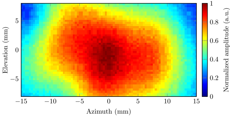
Figure 4.14: Beam profile hydrophone measurements of the fabricated linear transducer array prototype. The time signals were recorded at an axial distance of 107 mm with respect to the array.
