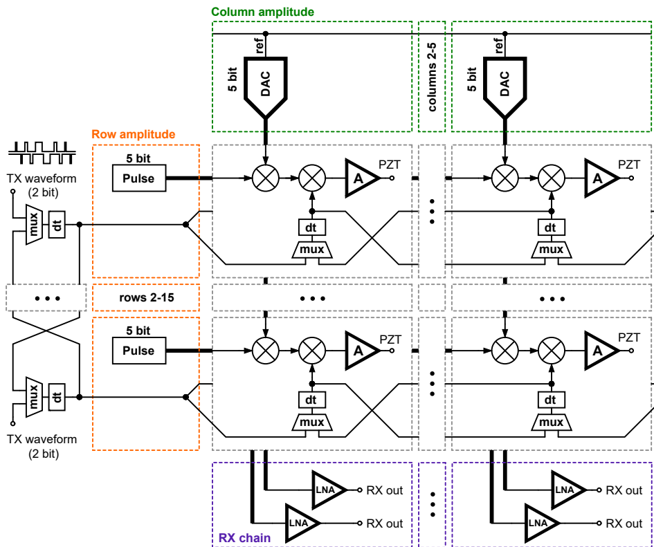
Figure 6.4: Block diagram of the prototype ASIC.
