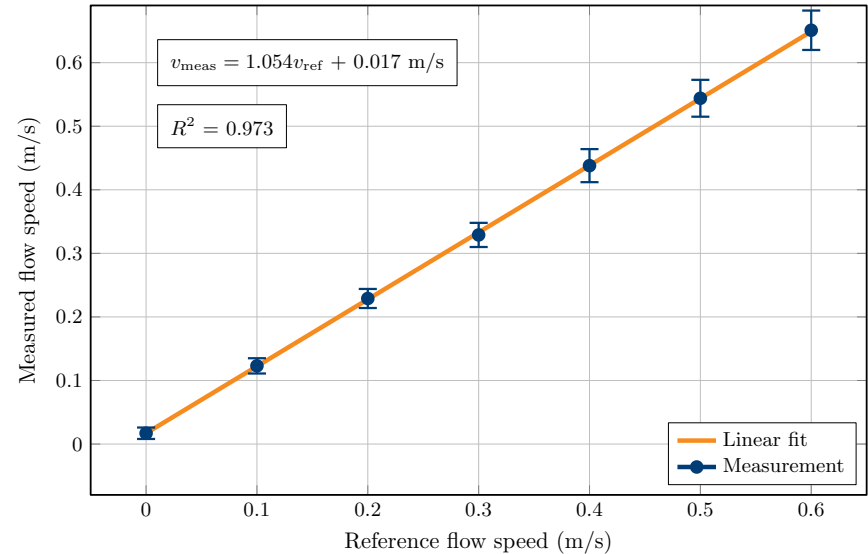
Figure 5.11: Measured and reference flow speed of water considering shear waves in the pipe wall. The vertical bars indicate median absolute deviations.
