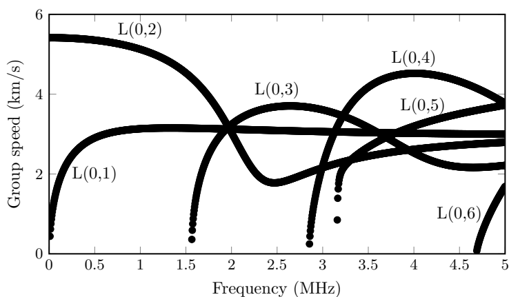
Figure 8.12: Group speed dispersion curves of Lamb waves for the pipe. Around 2.25\text{ MHz} , at least three different wave modes are expected to be excited.
