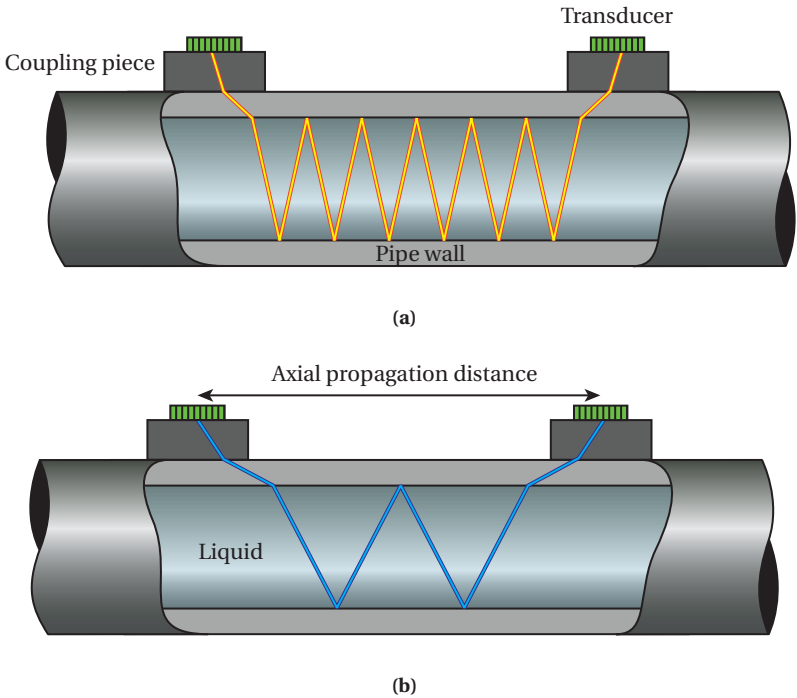
Figure 4.5: Travel path of an acoustic beam during ultrasonic clamp-on flow measurements using (a) compressional, and (b) shear waves in the pipe wall.
