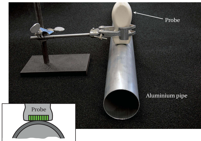
Figure 8.16: Experimental setup to test the proposed procedure for measurement of the pipe diameter, consisting of an aluminium pipe ( OD = 60\text{ mm} , h = 1\text{ mm} ), and a P4-1 phased array probe placed on top. The array elements of the probe are oriented perpendicularly to the pipe axis, as indicated by the diagram. A foam layer was placed below the pipe to avoid mechanical coupling and vibrations of the table on which the setup was placed.
