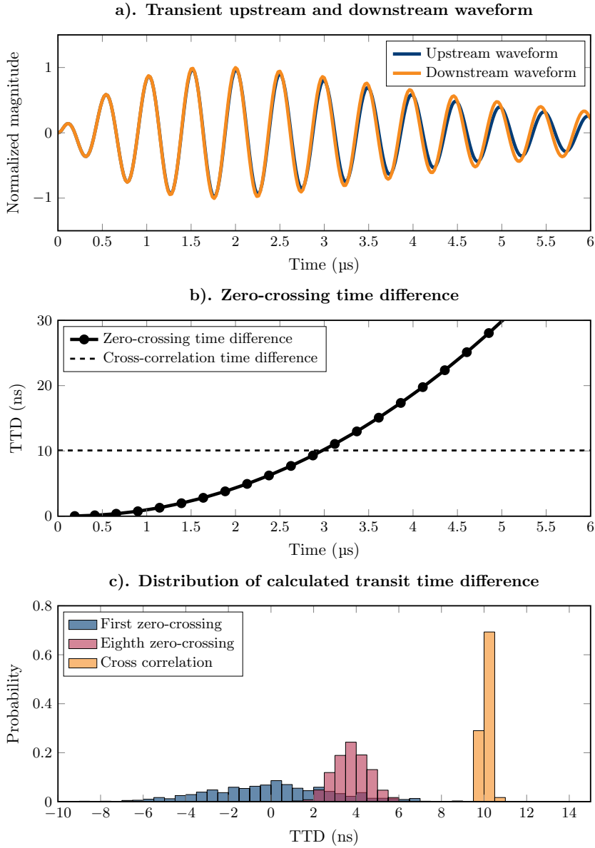
Figure 3.2: Simulated upstream and downstream signals for R_{\text{TX}} = 50\ \Omega and R_{\text{TX}} = 20\ \Omega , excited with a single square pulse: a). Transient waveforms, b). Upstream-downstream time-difference (markers represent zero-crossings) and c). Probability distribution of the transit-time difference obtained using the zero-crossing and cross-correlation based algorithms for 2000 simulated waveforms with 30 dB SNR.
