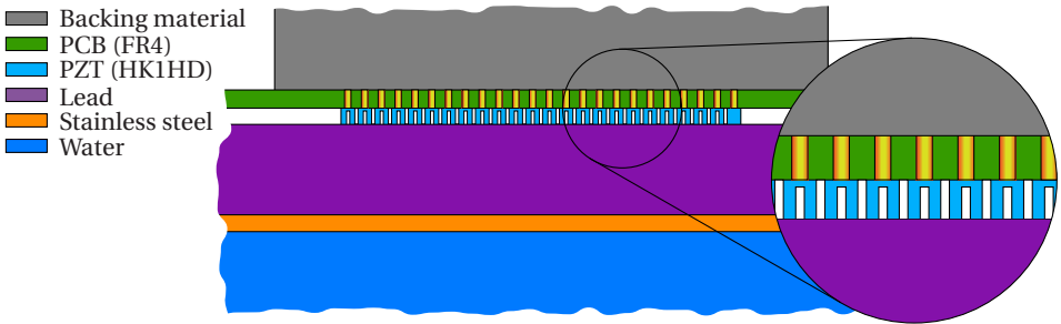
Figure 4.8: Acoustic stack of the designed transducer array. The sub-dicing kerfs of the PZT elements run up to 95 % of the element thickness. The vias in the PCB are 200 \mu\text{m} diameter and their walls are covered by a 20 \mu\text{m} thin copper layer.
