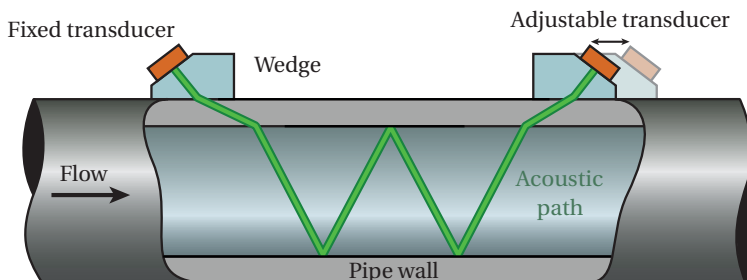
Figure 6.1: Diagram of a clamp-on ultrasonic flow meter.
