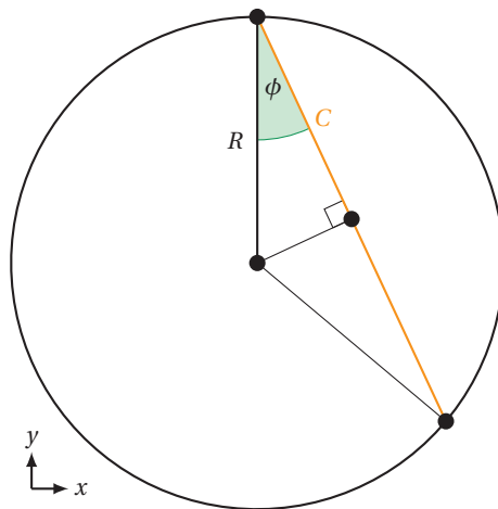
Figure 9.2: Calculation of acoustic path line integral (cross-sectional projection).
