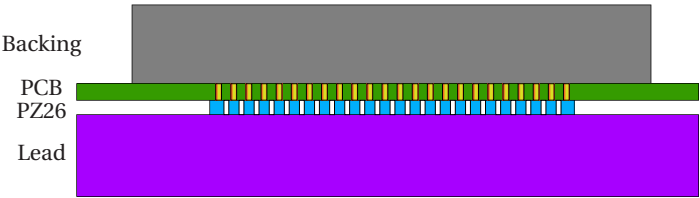
Figure 4.11: Geometry of the fabricated linear transducer array prototype. The PCB included air-filled vias with a diameter of 200\text{ }\mu\text{m} and a 20\text{ }\mu\text{m} -thick copper layer on the sides.
