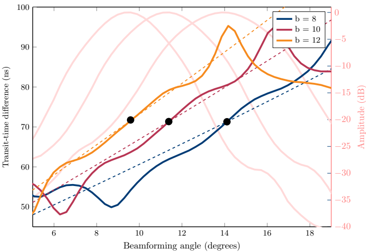
Figure C.2: Influence of the beamforming angle on the transit-time difference for three acoustic paths, simulated using ray-tracing. The dashed lines indicate the transit-time difference calculated using the approximated acoustic path length with equation (C.2). The black markers indicate the optimal steering angle (maximum signal amplitude).
