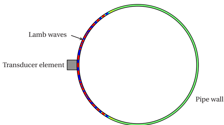
Figure 8.11: Finite Element simulation of an aluminium pipe ( OD = 60\text{ mm} , h = 1\text{ mm} ). The transducer element was excited with a 2-cycle sine wave with a center frequency of 2.25\text{ MHz} , and receivers were placed around the outer surface of the pipe wall. Transducer element dimensions ( 0.5 \times 0.3\text{ mm} ) are exaggerated for visualization purposes.
