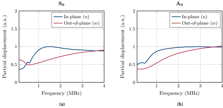
Figure 7.3: Amplitudes of the particle displacement of the zero-order Lamb waves in a 5 mm-thick stainless steel plate, loaded by water on one side, and by vacuum on the other side. A transducer array, placed on the vacuum-loaded surface of the plate, was used to excite an acoustic beam that impinged the steel-water interface with an angle of 45^\circ . The displacements u(\omega, x, z_0) and w(\omega, x, z_0) were computed across the thickness of the pipe wall ( -h \leq x \leq h ), at a propagation distance ( z_0 ) located at the edge of the transducer array.
