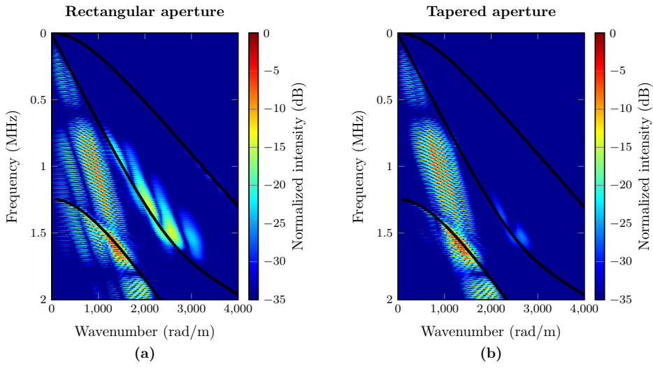
Figure 7.13: Normalized 2D FFT of the recorded space-time signals in Figure 7.12. The black lines represent the theoretical dispersion curves of the Lamb waves that propagate within the steel.
