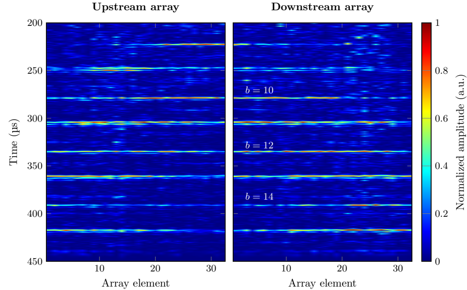
Figure 6.16: Acoustic signals of the upstream and downstream array, obtained in a single flow measurement. The wavefronts arriving via several acoustic paths can be observed.
