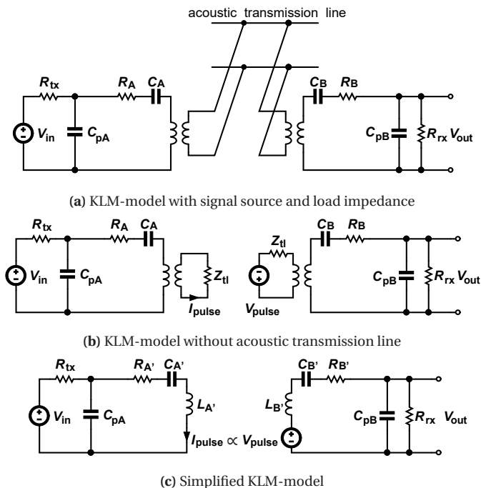
Figure 3.1: Simulation model based on simplified KLM-model.
