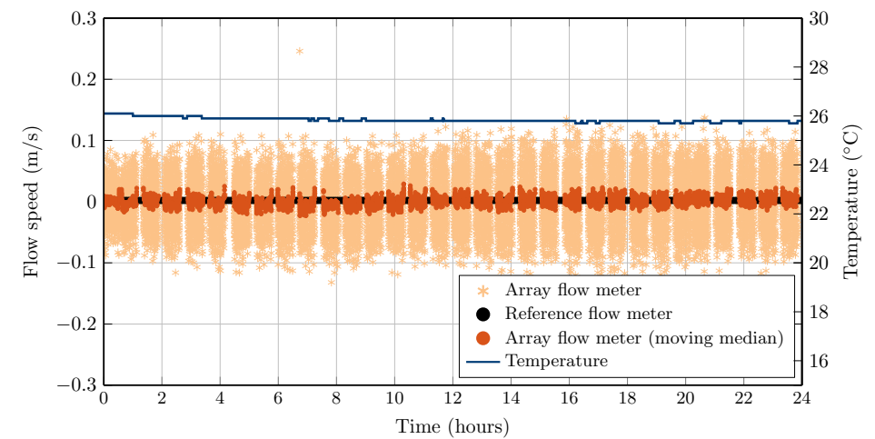
Figure 5.12: 24h-monitoring of the flow speed at zero-flow conditions, measured with the fabricated sensor considering a compressional wave in the pipe wall. Reference flow speed measurements are shown in black, and a temperature log of the water is shown in blue. A moving median of the measured flow speeds with the fabricated sensor is shown in orange, considering a time window of 300 points (i.e. 5 min).
