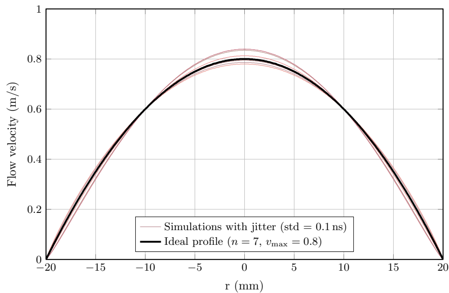
Figure 9.6: Estimation of velocity profiles with simulated data for 10 flow measurements with a jitter of 0.1 ns and laminar flow with v_{\text{max}} = 0.8 m/s.
