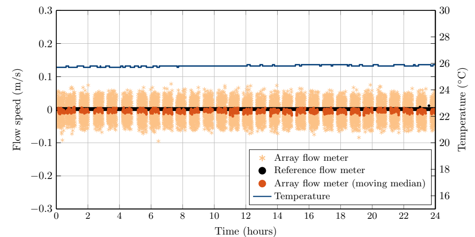
Figure 5.13: 24h-monitoring of the flow speed at zero-flow conditions, measured with the fabricated sensor considering a shear wave in the pipe wall. Reference flow speed measurements are shown in black, and a temperature log of the water is shown in blue. A moving median of the measured flow speeds with the fabricated sensor is shown in orange, considering a time window of 300 points (i.e. 5 min).
