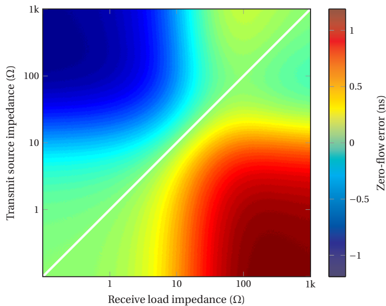
Figure 2.4: Simulation of the zero-flow error based on an upstream and downstream measurement with 10 % mismatch in C_m of the transducer model. The diagonal white line highlights equal transmit and receive impedances.
