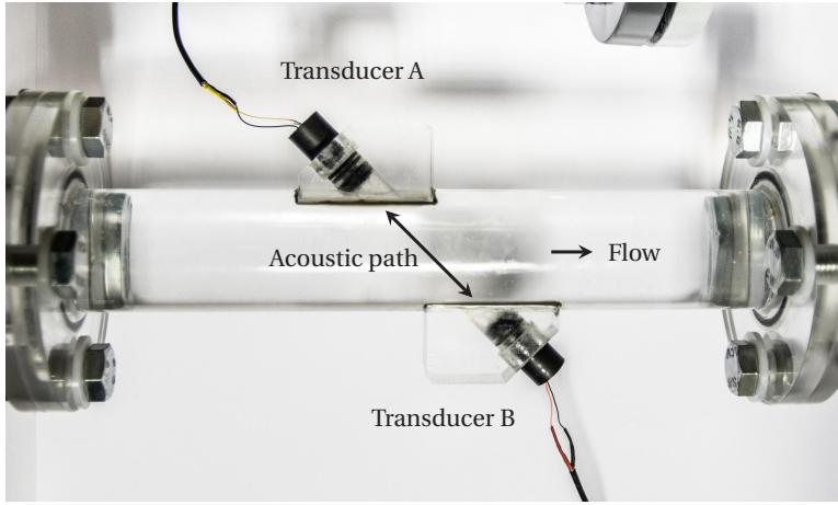
Figure 3.5: Transducers placed co-axially at a 45^\circ angle in a 40 mm inner-diameter pipe section of the flow-loop.
