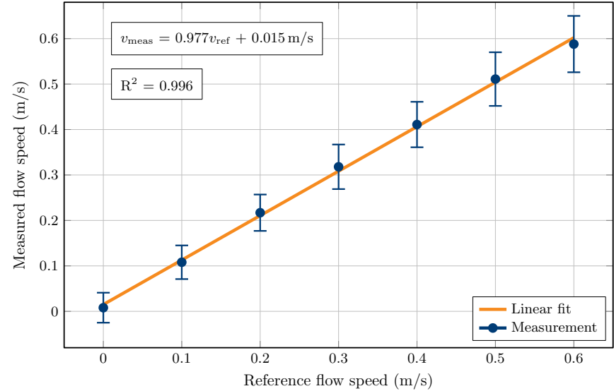
Figure 5.10: Measured and reference flow speed of water considering a compressional wave in the pipe wall. The vertical bars indicate median absolute deviations.
