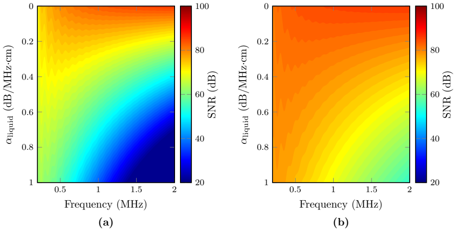
Figure 4.10: Computed SNR of the designed transducer array versus frequency and attenuation coefficient of the liquid for compressional waves in the pipe wall and six bounces within the pipe (a) and shear waves in the pipe wall and two bounces within the pipe (b).
