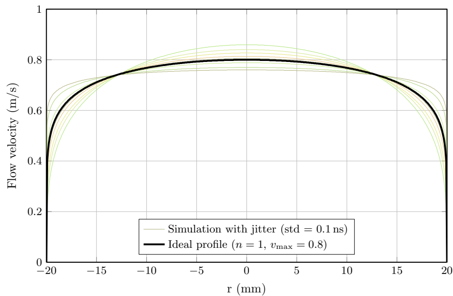
Figure 9.7: Estimation of velocity profiles with simulated data for 10 flow measurements with a jitter of 0.1 ns and turbulent flow with v_{\text{max}} = 0.8 m/s.
