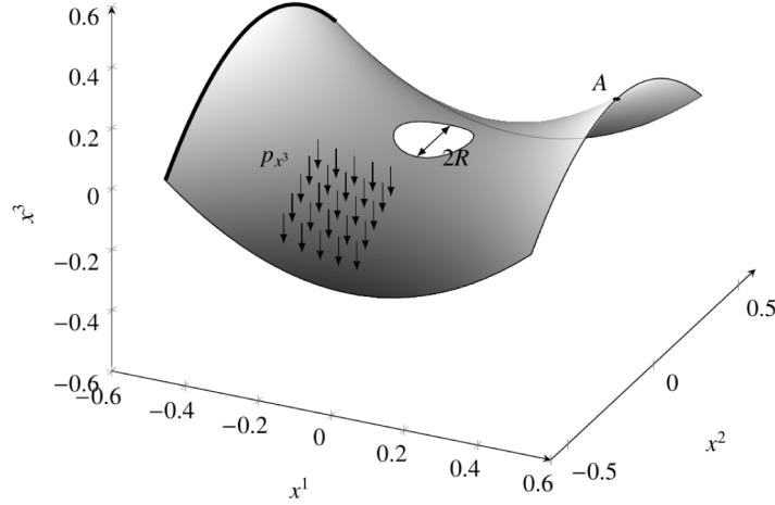
Fig. 6. Set-up of the clamped hyperboloid with a hole of radius R = 0.15 . The displacements and rotations are fixed on the left boundary represented by the thick line. The distributed load p_{x^3} is applied over the whole domain in vertical direction. Furthermore, the point A is used for reference.
