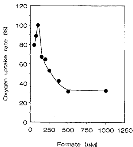
FIG. 2. Oxidation of formate by T. ferrooxidans cells: effect of substrate concentration. Formate-dependent oxygen uptake rates were measured at 30°C with cell suspensions taken directly from a formate-limited chemostat culture ( D = 0.01 \text{ h}^{-1} , pH 1.8, 30°C). An activity of 100% corresponds to an oxygen uptake rate of 55 nmol of O 2 · min -1 · mg -1 .
