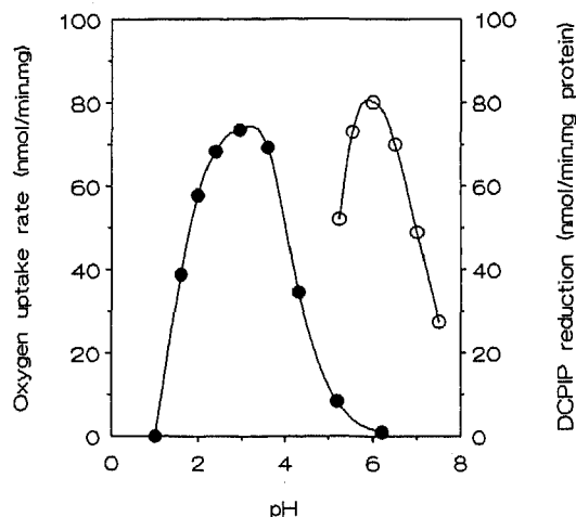
FIG. 3. Oxidation of formate by cell suspensions (●) and cell extracts (○) of T. ferrooxidans : effect of pH. Formate-dependent oxygen consumption rates were measured with cell suspensions from a formate-limited chemostat culture ( D = 0.01 \text{ h}^{-1} , pH 1.8, 30°C). Suspensions were adjusted to the appropriate pH by the addition of dilute H 2 SO 4 or KOH. Oxidation of formate by cell extracts was assayed as formate-dependent reduction of DCPIP (see Materials and Methods).
