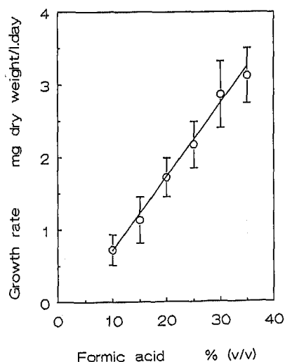
FIG. 1. Growth of T. ferrooxidans on evaporated formate in adapted Erlenmeyer flasks (pH 2.0, 30°C): effect of formate concentration in the reservoir on the growth rate. Independent, triplicate cultures were inoculated with cells from formate-limited chemostat cultures ( D = 0.01 \text{ h}^{-1} , pH 2.0, 30°C). Dry weights were estimated from the optical densities of the cultures by using calibration curves made with formate-limited chemostat cultures.
