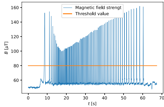
Figure 2. The raw data recorded using the Phyphox app, magnetic field strength as a function of time.
