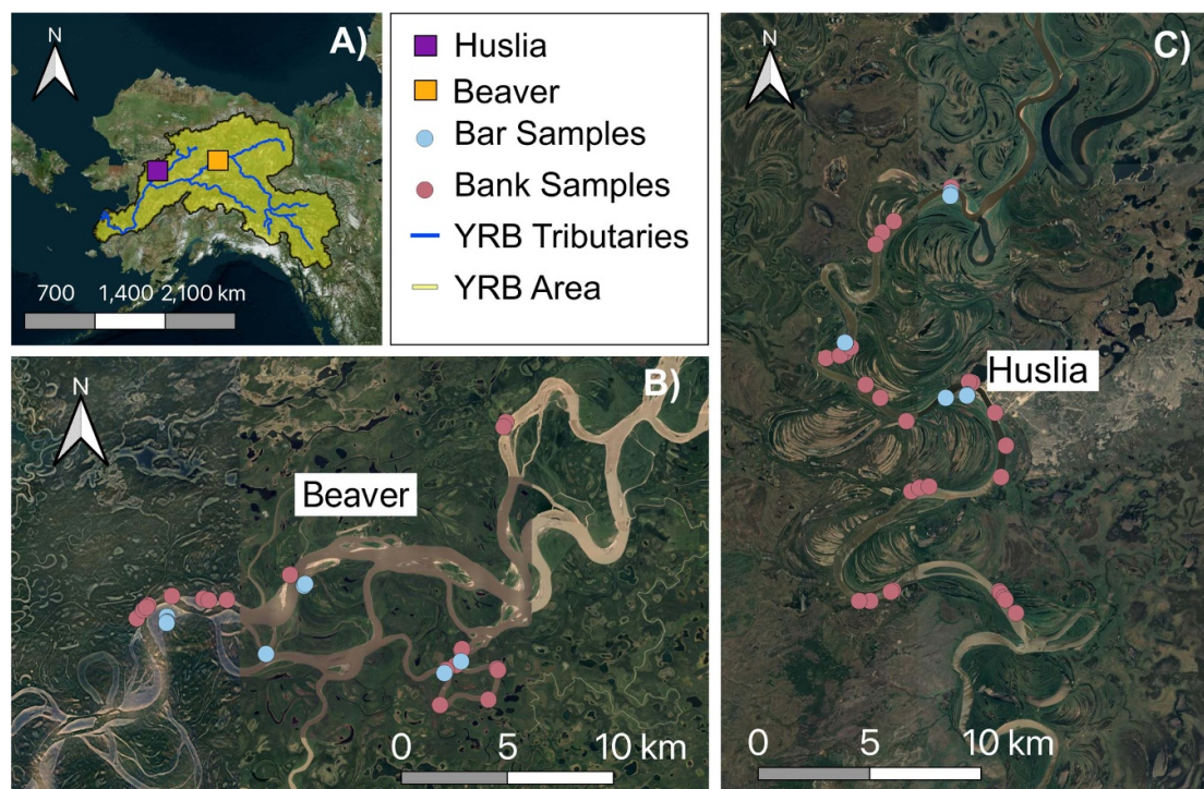
Figure 1. Study sites located in interior Alaska in the YRB (watershed boundary-yellow shaded region [34], tributaries-blue line) (A). Samples were collected along an anastomosing, gravel-bedded reach of Yukon River (B) and a sand-bedded reach of the Koyukuk River (C), a single-threaded meandering river that is a major tributary of the Yukon River. Sampling locations were located near the villages of Huslia (purple square in A) and Beaver (orange square in A). Dots represent cutbanks (red; n = 56 ) and point bars (blue; n = 29 ) that have been characterized. Samples were collected in June 2022 (Huslia: 18 cutbanks, 6 point bars; Beaver: 13 cutbanks, 6 point bars) and September 2022 (Huslia: 15 cutbanks, 8 point bars; Beaver: 10 cutbanks, 6 point bars) (supplementary, dataset S1). To capture a holistic view of the floodplain, sites were selected to span a range in ages, terrain type, and permafrost presence determined from geomorphic maps [33, 35, 36]. Seasonal variation in water level affected sampling site accessibility, so sites from June and September are complimentary, but not identical.] (A) Microsoft® Bing™ Maps Platform screen shot(s) reprinted with permission from Microsoft Corporation [37]. Yukon River Watershed Boundary shapefile reproduced [34] with permission from Yukon River Inter-Tribal Watershed Council. (B) and (C) Map data: Google, Maxar Technologies, CNES/Airbus, Landsat/Copernicus [38].
