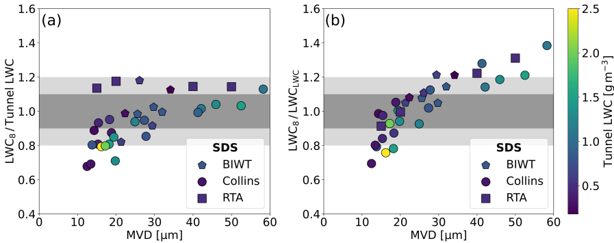
Figure 4.16: Comparison of the collision efficiency corrected 8 mm cone measurements ( \text{LWC}_8 ) to the tunnel LWC (a) and to the collision efficiency corrected LWC sensor measurements ( \text{LWC}_{\text{LWC}} ) (b).
