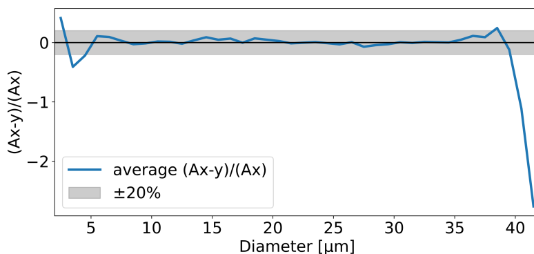
Figure 4.22: Average values of the normalized residuals between the elements of \mathbf{Ax} and \mathbf{y} , shown here for BCPD test point 407.
