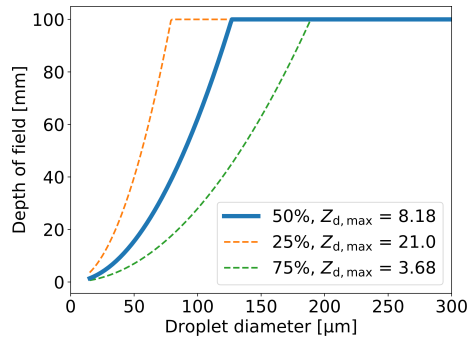
Figure 3.17: Depth of field of a CIP grayscale probe for different droplet diameters and a shadowing threshold of 50%, the DoF curves for 25% and 75% shadowing are shown for comparison. The Z_{d,max} values were taken from Korolev et al. [72]. A laboratory calibration of the DLR-CIP yielded the same Z_{d,max} value for 50% [73]. No measurements of the 25% and 75% threshold were performed at DLR. The arm width of the CIP is 100 mm and thus represents a mechanical limit to the DoF for all shadowing thresholds.
