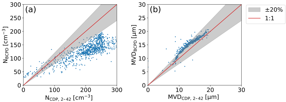
Figure 5.14: Comparison of the number concentration ( N ) (a) and the median volume diameter (MVD) (b) measured by the Cloud Droplet Probe (CDP) and the Backscatter Cloud Probe with Polarization Detection (BCPD) during predominantly liquid segments of the research flight.
