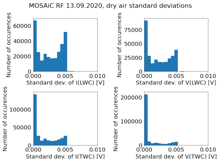
Figure A.4: Histogram of the standard deviations of the current (I) and the voltage (V) measured by the Nevzorov LWC sensor (top row) and by the Nevzorov 8 mm cone (bottom row) during two-second intervals in dry air.
