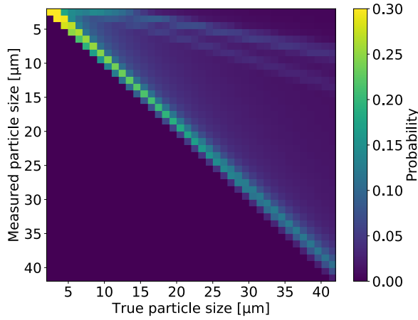
Figure 4.21: The Matrix \mathbf{A} that describes the measurement behavior of the Backscatter Cloud Probe with Polarization Detection.
