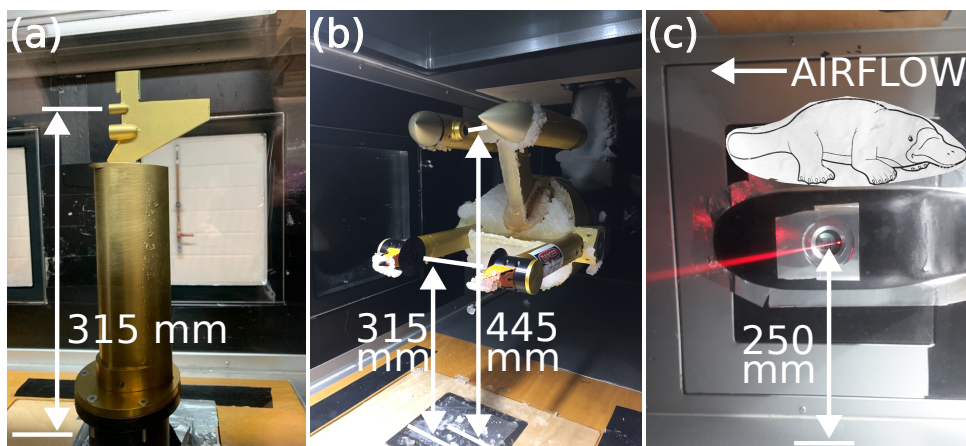
Figure 4.3: Mounting positions of the Nevzorov probe (a), CCP (b) and BCPD (c) in the Braunschweig Icing Wind Tunnel.
