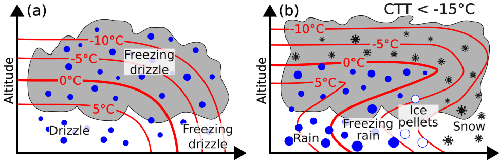
Figure 2.1: Formation of freezing drizzle through the supercooled warm rain process (a) and of freezing rain through the cold rain process (b). Cloud top temperatures (CTTs) are usually above -15\text{ }^{\circ}\text{C} for freezing drizzle formation and below -15\text{ }^{\circ}\text{C} for freezing rain formation. Image based on Marwitz et al. [14].
