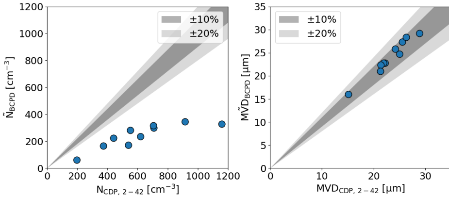
Figure 4.18: Comparison of the number concentrations (N) (a) and median volume diameters (MVDs) (b) measured by the Cloud Droplet Probe (CDP) and the Backscatter Cloud Probe with Polarization Detection (BCPD). The tilde symbol above the BCPD parameters signifies that no correction for undersizing effects (see Section 4.4.2) has been applied. The subscript 2-42 for the CDP parameters specifies that the size range for the CDP has been adjusted to match that of the BCPD.
