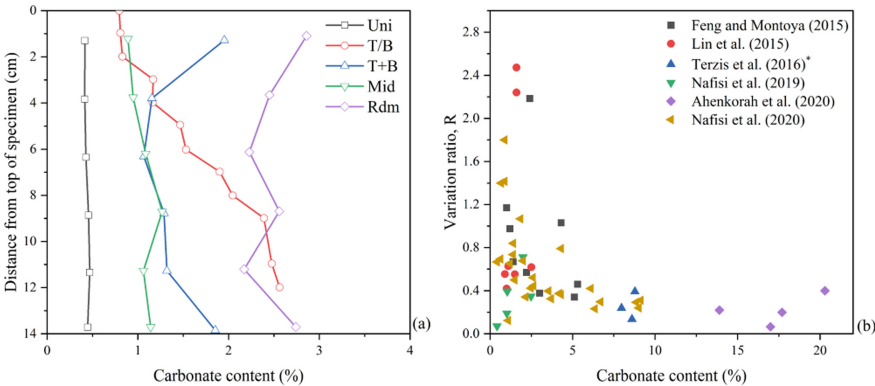
Fig. 1. (a) Illustration of spatial distribution type of carbonate content, data of uniform type, type Mid and type Rdm are cited from Nafisi et al. (2019), data of type T/B is cited from Lin et al. (2015), data of type T + B is cited from Nafisi et al. (2020). (b) Review on variation ratio of experimental data. *Note that carbonate content in Terzis et al. (2016) is defined as the mass of carbonate divided by the total mass of carbonate and sand.
