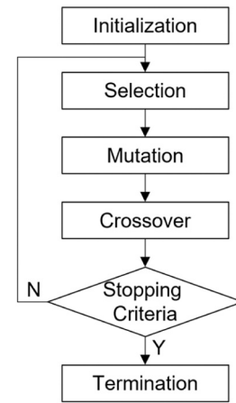
Fig. 2. Scheme of genetic algorithm.
