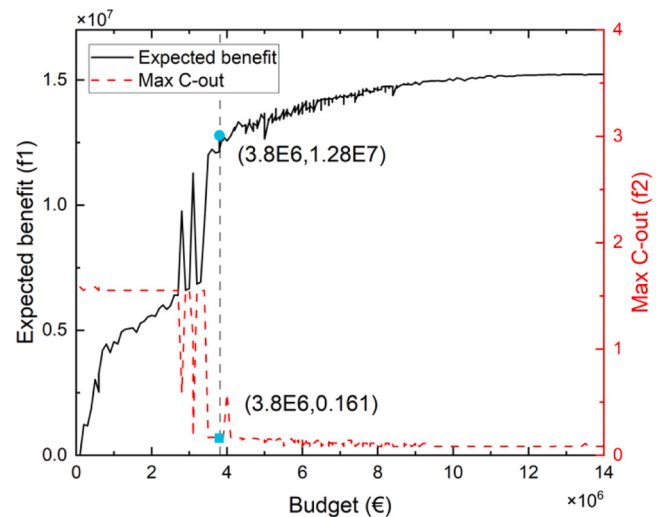
Fig. 7. Variation trends of two objective functions in Case 1.
