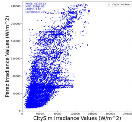
Figure 8. Scatter Plot of Monthly Solar Irradiance Values in Maastricht between Perez model results and CitySim results using the EPW as input weather data
