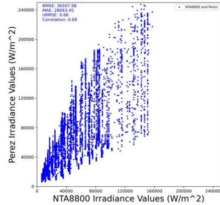
Figure 7. Scatter Plot of Monthly Solar Irradiance Values in Utrecht between Perez model results and NTA8800 using the EPW as input weather data
