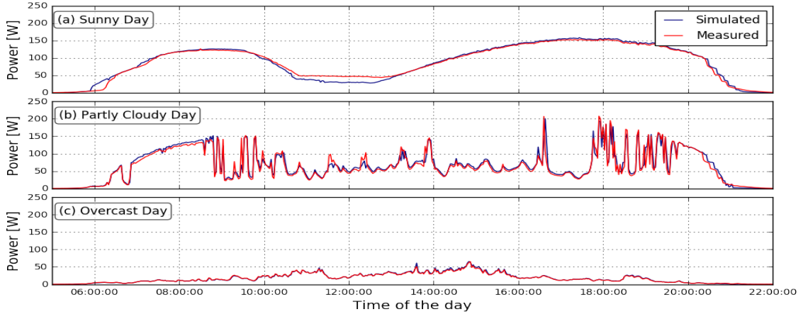
Figure 4: Simulated and measured power output during (a) sunny day, (b) partial cloudy day, (c) overcast day.
