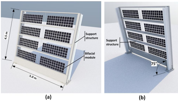
Figure 1: Computer rendering of one section of bifacial photovoltaic noise barrier containing 4 \times 2 modules, each with 4 \times 12 cells of 15 \times 15 cm. Front view (a) and rear view (b).
