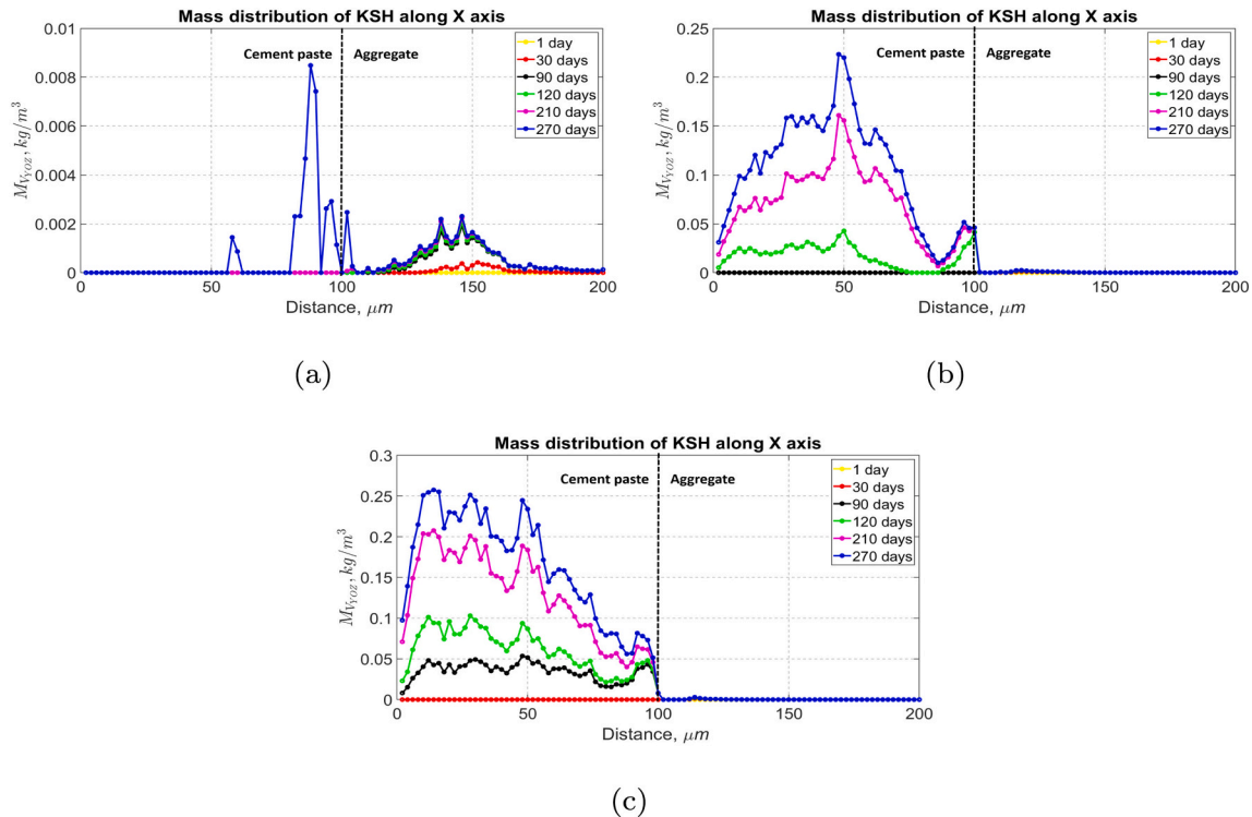
Fig. 10. The mass distribution evolution of KSH along X axis represented by M_{V_{YOZ}} in systems with different reactive silica contents in aggregate. (a): in system A_{31} with 6.58% reactive silica content; (b): in system A_{33} with 20.51% reactive silica content; (c): in system A_{35} with 40.91% reactive silica content.
