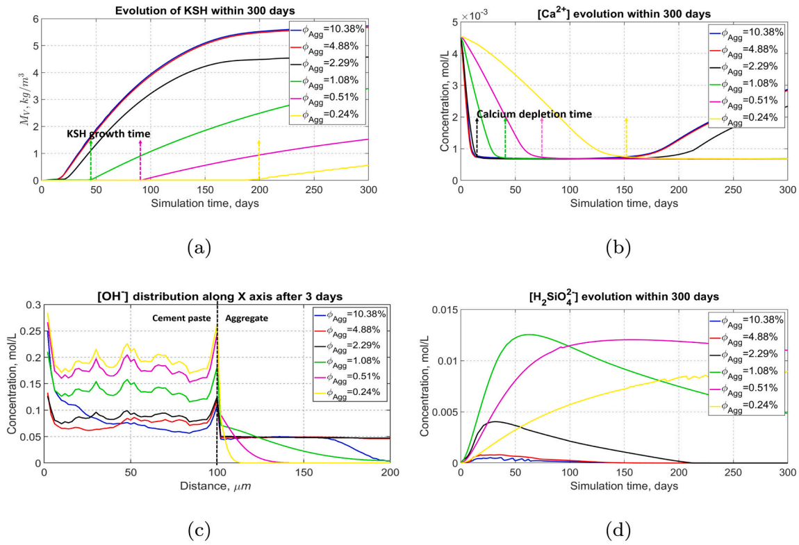
Fig. 7. (a): Mass evolution of KSH represented by M_V in systems with different aggregate porosity within 300 days; (b): The concentration evolution of Ca 2+ in systems with different aggregate porosity within 300 days; (c): Distribution of average concentration of OH - along X axis in systems with different aggregate porosity after 3 days; (d): The concentration evolution of H 2 SiO 4 2- in systems with different aggregate porosity within 300 days.
