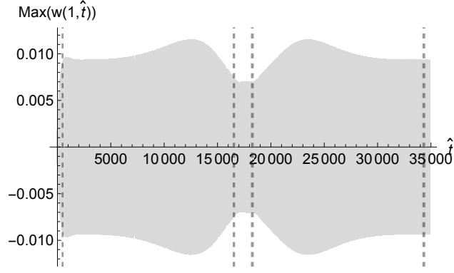
Figure 5: Time response of the beam during linear motion when \hat{Z} = 0.000015 and \hat{\omega} = 3.268 . The moving particle has M = 20pg and a velocity of 0.004m/s . The time history is evaluated for the complete travel of the particle inside the two legs of the beam.
