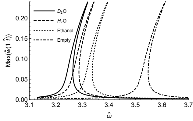
Figure 9: Influence of fluid on the non-linear frequency response curves ( \hat{Z} = 0.0003 ). — beam filled with deuterium oxide ( \rho_{D_2O} = 1100\text{kg/m}^3 ), --- water ( \rho_{H_2O} = 1000\text{kg/m}^3 ), -.-.- empty beam, ..... channel filled with Ethanol ( \rho_{EtOH} = 790\text{kg/m}^3 ).
