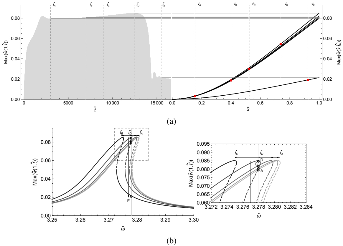
Figure 10: Maximum deflection of the beam under the action of the moving particle when the excitation frequency and amplitude are fixed at \hat{\omega} = 3.278 and \hat{Z} = 0.00011 , and particle velocity is 0.004\text{m/s} . Points A-E depict different time instants at which the particle lies at specific position along the channel. (a) Time response along one leg of the beam with the corresponding maximum deflection. (b). Frequency response curve translation due to the particle movement. The upper horizontal arrows indicate the translation of the resonant peak and dashed lines indicate unstable solutions.
