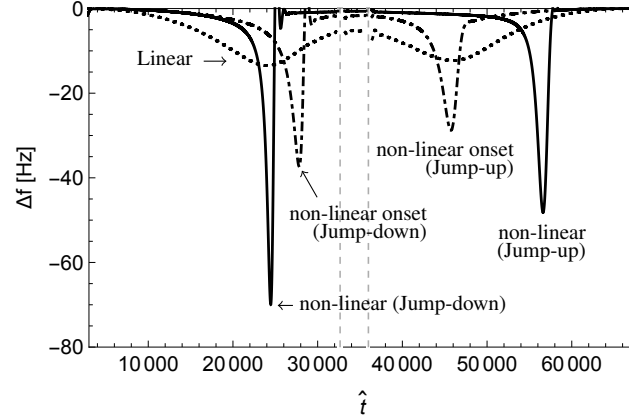
Figure 13: Frequency drop in time (full particle travel) for different excitation amplitudes and frequencies. --- \hat{Z} = 0.00003 - \hat{\omega} = 3.27 , -.-.- \hat{Z} = 0.00008 - \hat{\omega} = 3.273 , — \hat{Z} = 0.0001 - \hat{\omega} = 3.277 .
