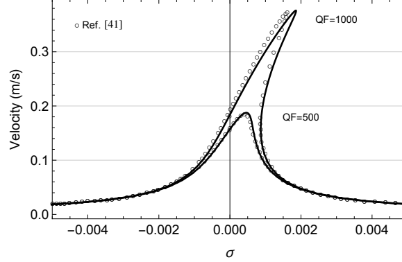
Figure 4: Comparison of the result presented in Figure 10(b) of Ref. [41] ( \circ ) with that replicated by means of the current model (solid line). For the simulations, three modes are retained in the discretization.
