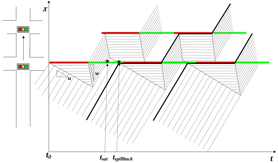
Figure 5 Trajectories of vehicles passing two intersections with spillback (The upstream intersection is under-saturated)
