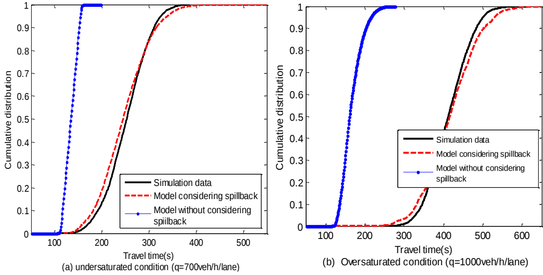
Figure 20 Comparison of travel time distributions (CDF) from VISSIM simulation and the proposed model considering and without considering spillback at 5 th cycle
