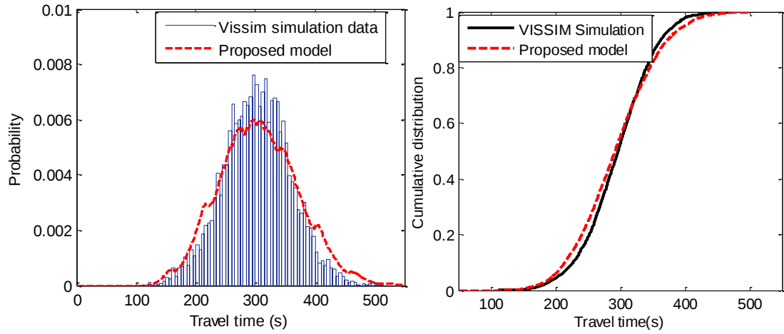
(b) With spillback (offset=25s)
