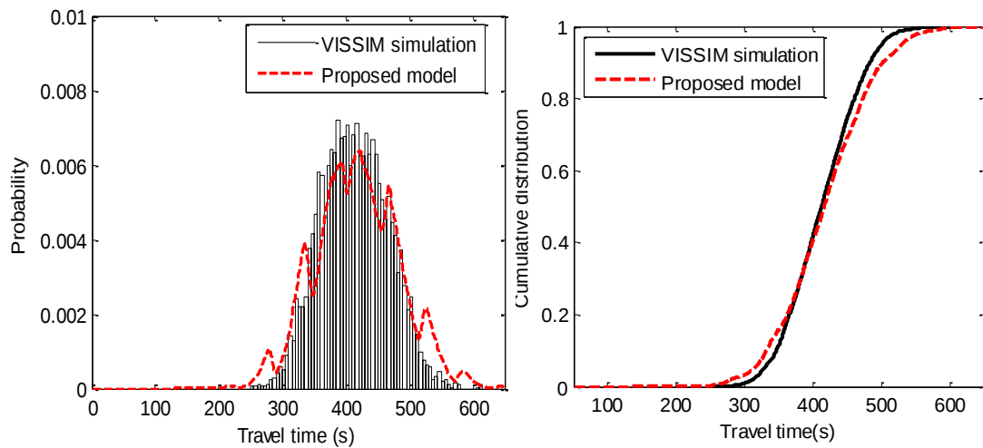
(b) With spillback (offset=25s)
