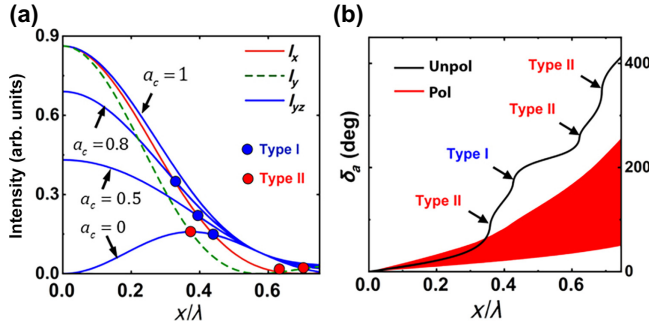
FIG. 4. (a) Focal intensities I_x (red) and I_{yz} (blue) for polarized illumination for different values of a_c ; I_y is shown, for reference, as the dashed green line. Type-I and II PISs are marked as blue and red dots, respectively. (b) Accumulated angular shifts for the singular points, under unpolarized illumination (black curve) and for the polarized case with a_c \in [0, 1] (red part).
