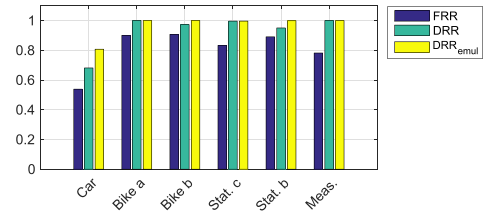
Fig. 18. Data recovery ratio (DRR) in emulation results for five datasets, using parameters R=1/2 , W=8 . 'Stat.' means stationary data. 'Bike b' and 'Stat. b' are bursty datasets. 'Meas.' is a new dataset acquired while using DaRe at runtime.
