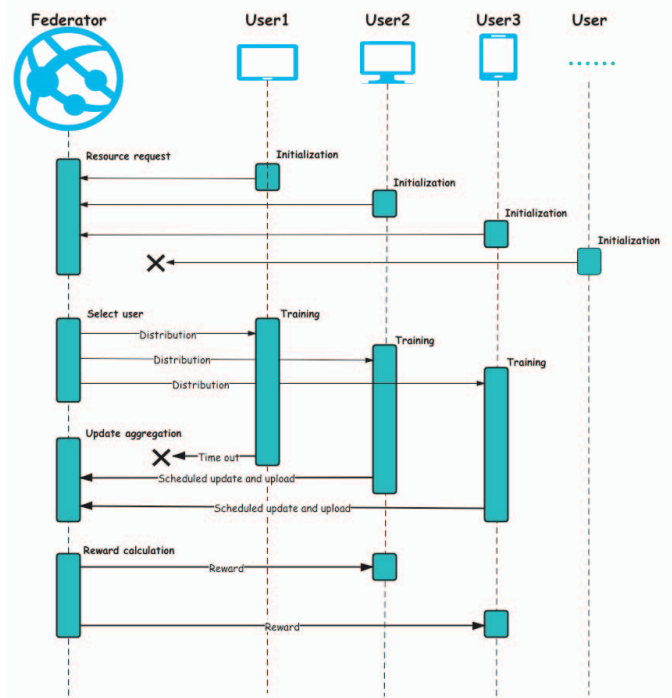
Fig. 2: Protocol of Federated Learning
