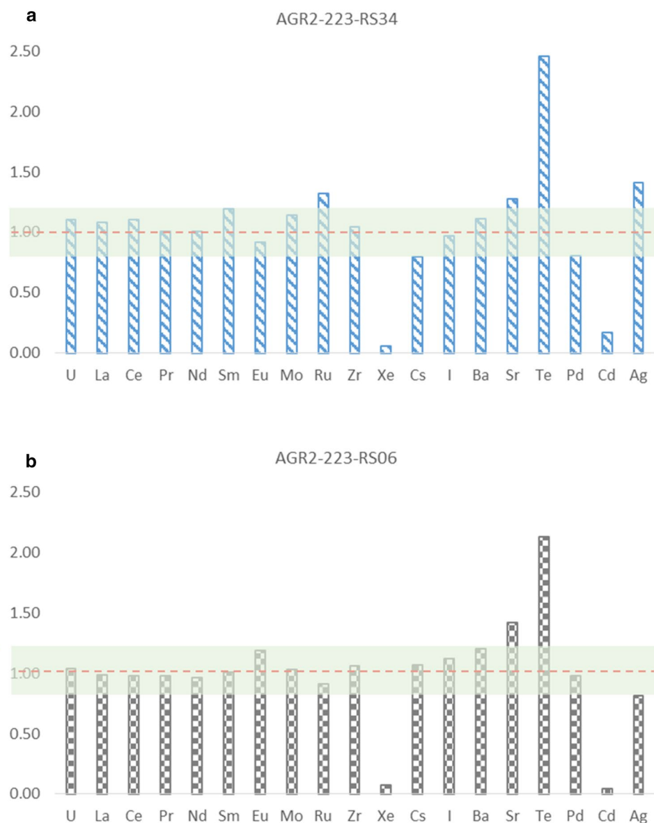
Fig. 2 a, b. Shows the ratio of the EPMA-calculated particle mass to the ORIGEN-predicted mass for U and 18 FPs in particle AGR2-223-RS34 ( a ) and particle AGR2-223-RS06 ( b ). The horizontal dotted line denotes a 1:1 ratio between calculated and predicted masses while the shaded box indicates the \pm 20\% calculated:predicted ratio region
