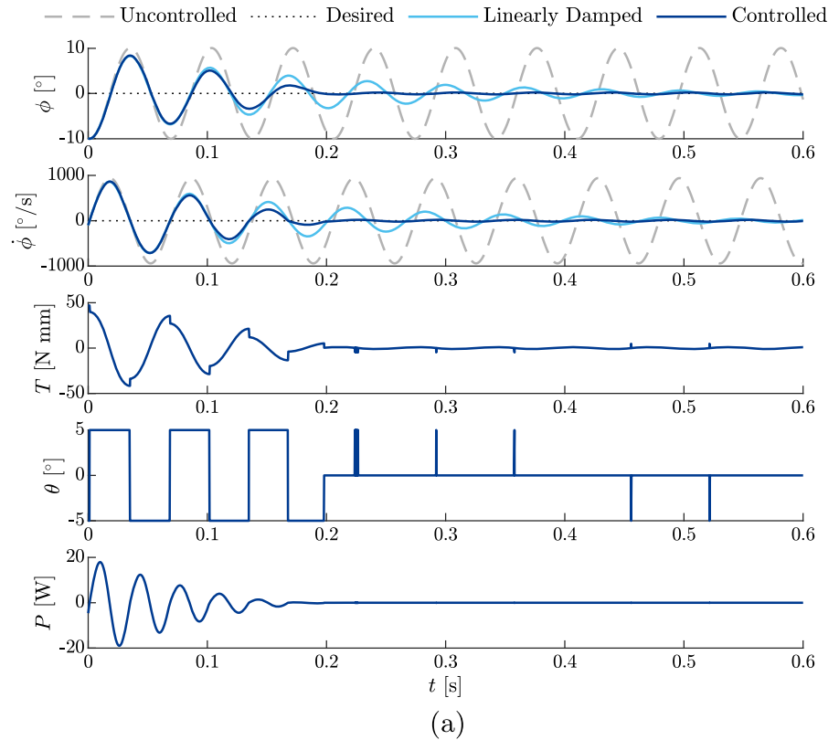
Fig. 5 Damping control system's response: a times series of the rotation \phi and the angular velocity \dot{\phi} of the ring, the actuation torque T , the orientation \theta , and the power of the magnetic interaction P , b phase portrait of the system's response in the damping control mode
