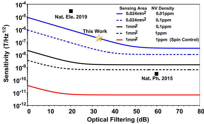
FIGURE 4. Estimation of sensitivity for hybrid CMOS-NV magnetometers [60].
