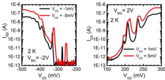
FIGURE 17. Measured minimum size 22-nm FDSOI p-MOSFET (SHT) and n-MOSFET (SET) transfer characteristics showing strong quantum effects at 2 K and large back-gate voltages and the impact of V_{DS} .
