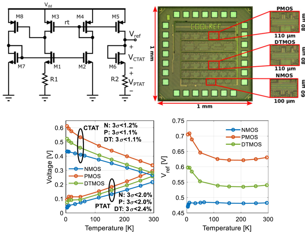
FIGURE 24. Voltage reference schematic and micrograph (Top) voltage stability performance (Bottom) of the CTAT and PTAT components (Left) and the output voltage (Right) [181].
