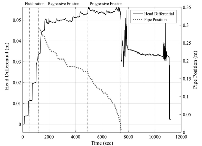
Fig. 6. Differential head (based on a projection of the 4 upstream [12–15] and 3 downstream [2–4] pressure transducers) and pipe y-position (distance from downstream end of the sample) for test B25-245.
