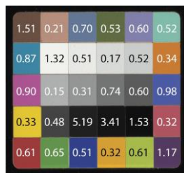
Figure 10: The color accuracy expressed with the \Delta E -2000 metric for each color patch of the ColorGauge Micro Target.
