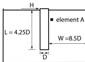
Fig. 23. Case example selected for the 3D FE simulation of cyclic MP tilt based on SANISAND-MS
