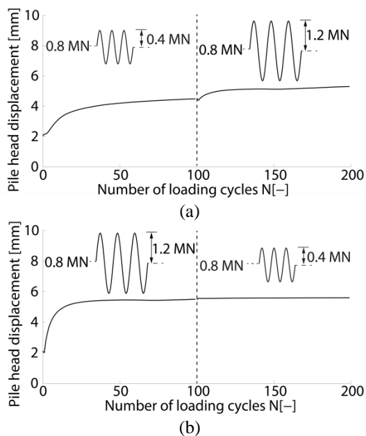
Fig. 24. Lateral displacement accumulation at MP head for cyclic load sequence (a) 1 and (b) 2 (Liu, 2020)
