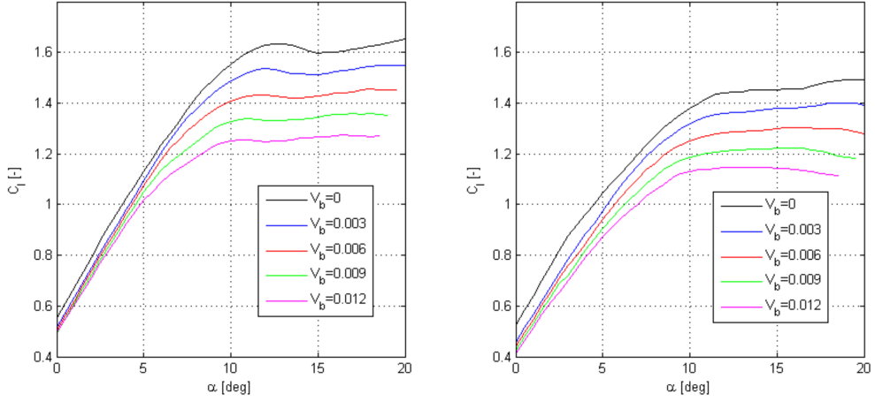
Figure 2.5: C_l vs \alpha for different blowing speeds V_b applied at x/c \in [0.05; 0.2] . Left - DU93 - W - 210 and Right - NACA64618
