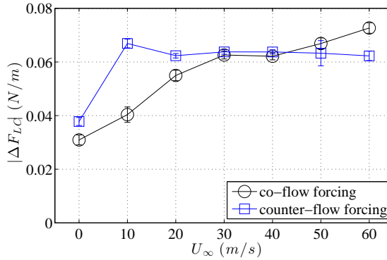
Figure 3.7: Measured force difference between actuator on and off .
