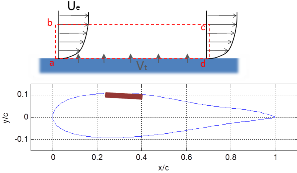
Figure 5.3: top - Equivalent Transpiration Control Volume - bottom - Airfoil Contour with indicated actuation
