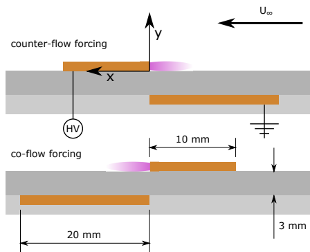
Figure 3.2: Geometrical configuration of the actuator in counter-flow and co-flow forcing configurations (not to scale).
