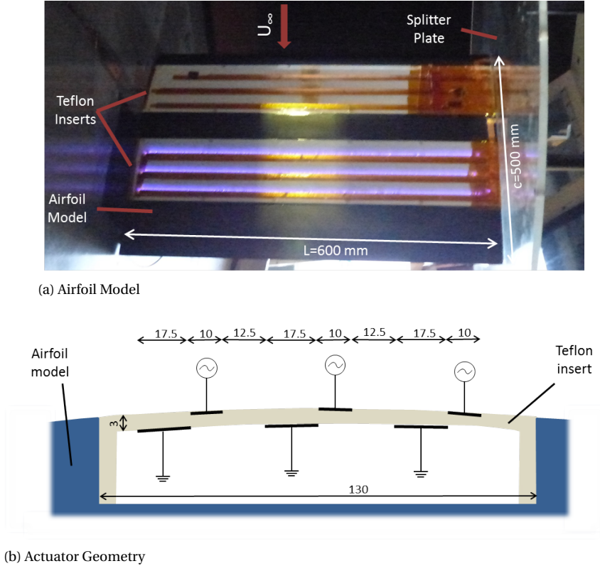
Figure 5.4: Experimental set-up
