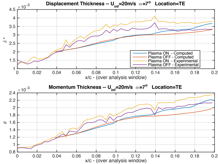
(b) TE actuation block at U = 20\text{m/s} and \alpha = 7\text{deg}
