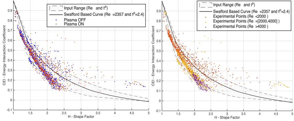
Figure 5.6: Energy Interaction Coefficient Comparison with Experimental Results - left - C_{EI} computation with and without plasma - right - C_{EI} computation over Re_\theta bins
