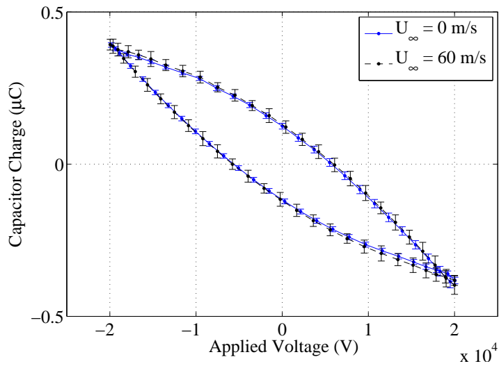
Figure 3.4: Lissajous curve for counter-flow forcing
