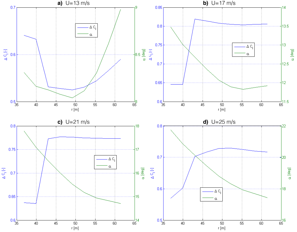
Figure 2.4: Required \Delta C_l and \alpha for different wind speeds, U = 13 m/s (a), U = 17 m/s (b), U = 21 m/s (c), U = 25 m/s (d)
