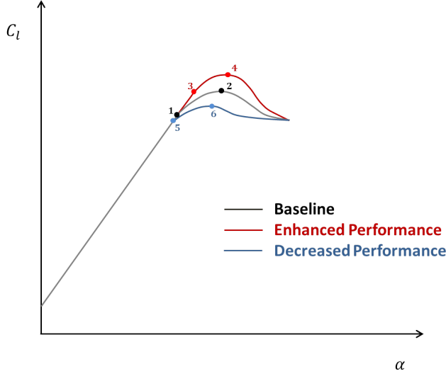
Figure 6.2: Example Baseline and Actuated Lift Polars
