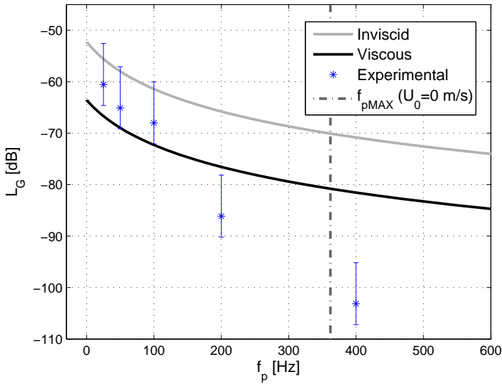
Figure 4.6: Modeled fluid system response, with experimental data from [71]- Influence of Viscosity in Quiescent case
