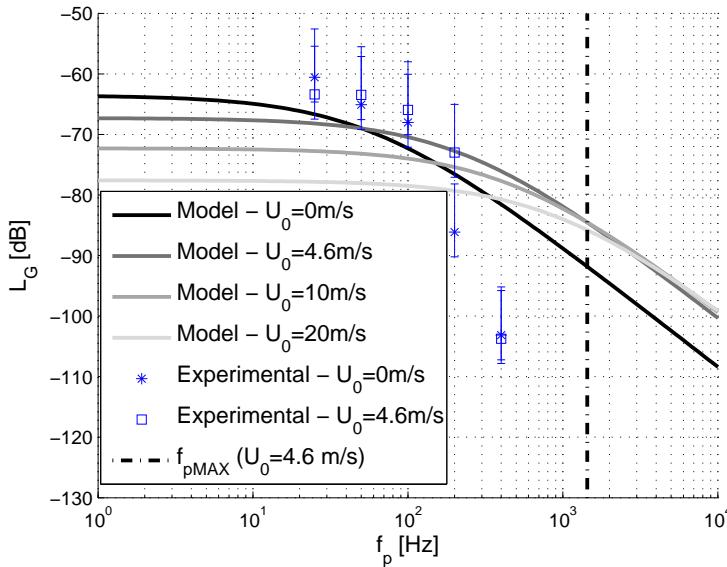
Figure 4.7: Modeled fluid system response, with experimental data from [71] - Influence of Velocity
