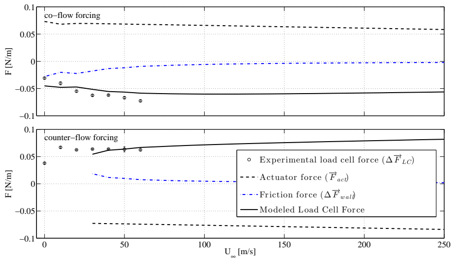
Figure 3.10: Model vs load cell results.
