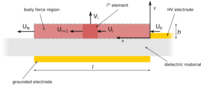
Figure 3.8: Computational model schematic for the co-flow forcing configuration.
