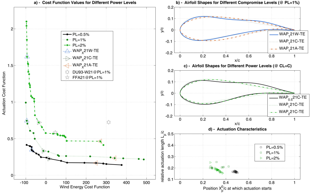
Figure 6.5: WAP - Transpiration Enhanced Performance - a) Cost Function Values, b) Compromise Level Shapes, c) Power Level Shapes, d) Actuation Characteristics
