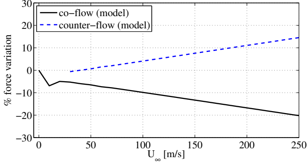
Figure 3.12: Modeled actuator force variation for different external flow speeds
