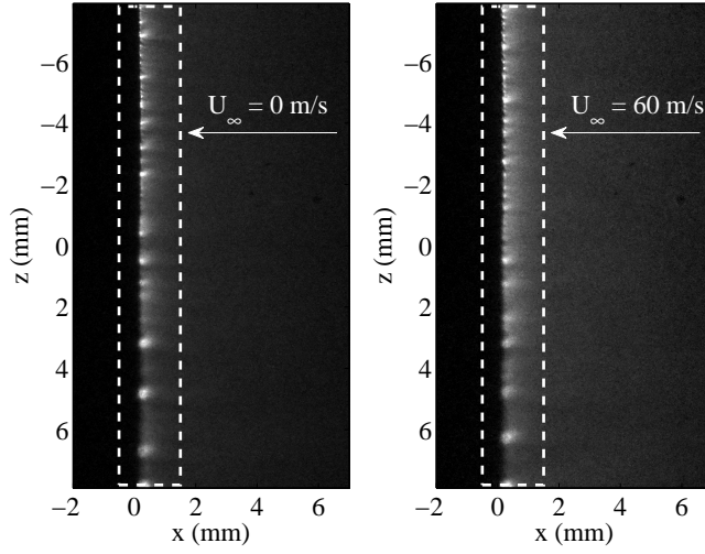
Figure 3.5: Light intensity of the discharge in counter-flow forcing configuration. White rectangle indicates the integration length for estimation of intensity (Fig.3.6).
