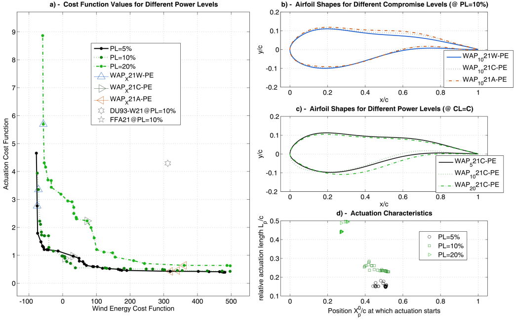
Figure 6.7: WAP - Plasma Enhanced Performance - a) Cost Function Values, b) Compromise Level Shapes, c) Power Level Shapes, d) Actuation Characteristics
