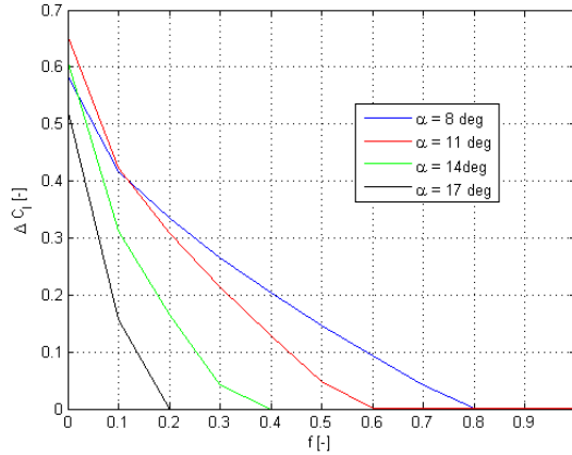
Figure 2.11: \Delta C_l vs f for different AOA - NACA64618 at Re = 10 \times 10^6
