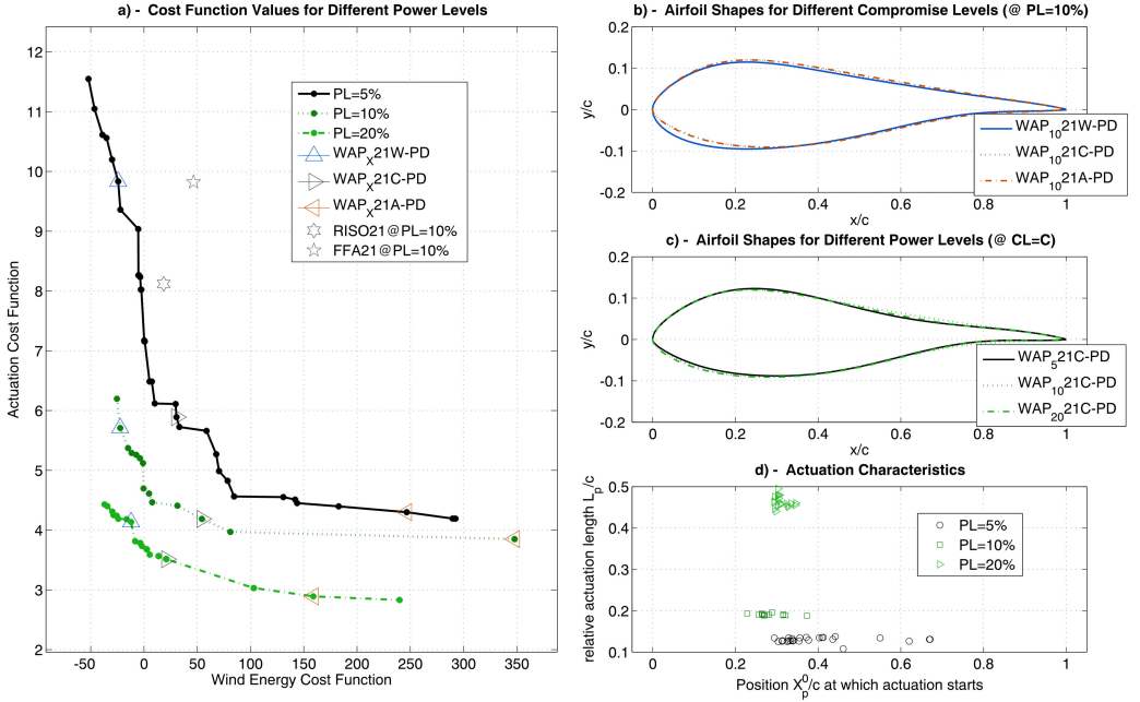
Figure 6.6: WAP - Plasma Decreased Performance - a) Cost Function Values, b) Compromise Level Shapes, c) Power Level Shapes, d) Actuation Characteristics
