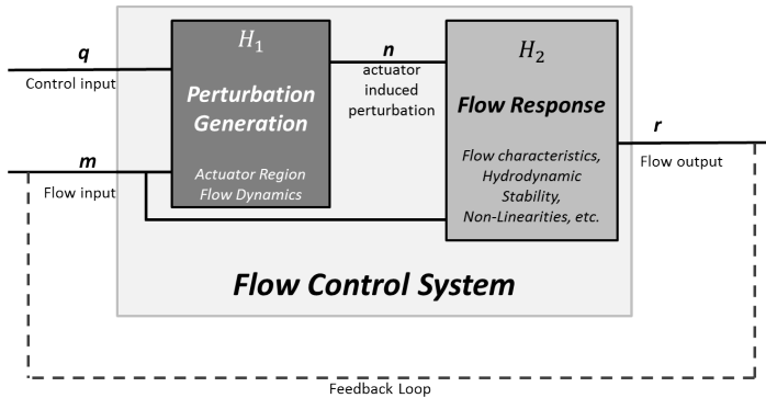
Figure 4.1: Illustration of subsystems in a flow control application
