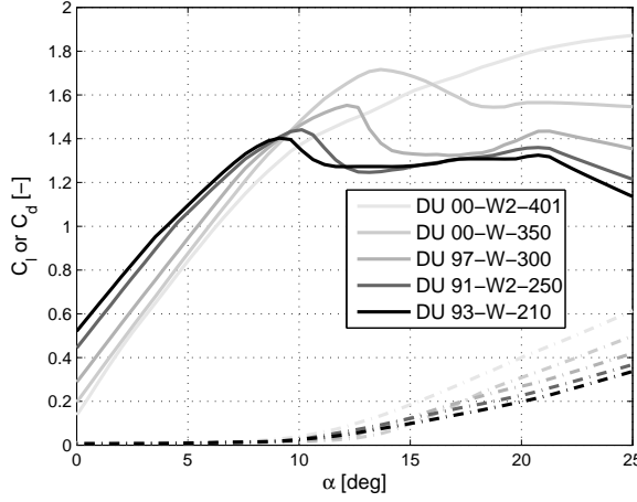
Figure 7.1: Aerodynamic Polars along blade span
