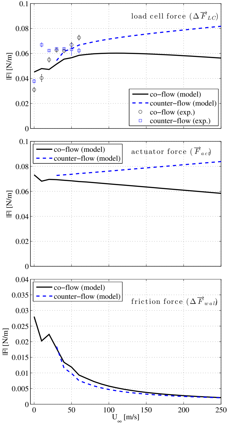
Figure 3.11: Individual absolute force terms for co-flow and counter-flow as predicted by the analytical model.
