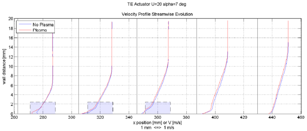
(c) velocity profiles
