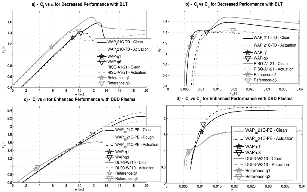
Figure 6.8: Airfoil Aerodynamic Polars - a) and b) Decreased Performance with BLT, c) and d) Enhance Performance with DBD Plasma
