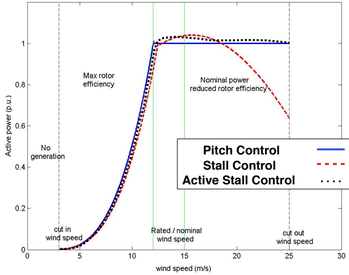
Figure 1.2: An example of different HAWT control strategies (adapted from [95])
