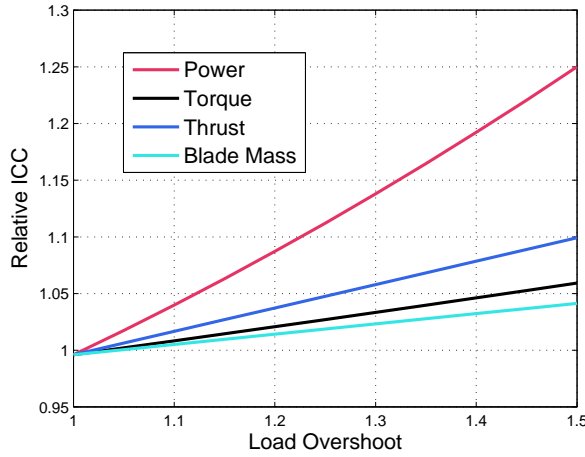
Figure 7.6: ICC Sensitivity to Different Load Overshoots
