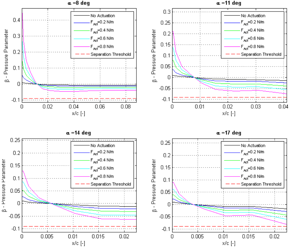
Figure 2.8: Laminar Separation Criteria as DBD actuation is applied for \alpha = [8; 11; 14; 17] at V_{eff} = 60 \text{ m/s}
