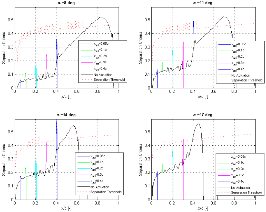
Figure 2.10: Turbulent Separation Criteria as DBD actuation is applied for \alpha = [8; 11; 14; 17] at V_{eff} = 60 \text{ m/s}
