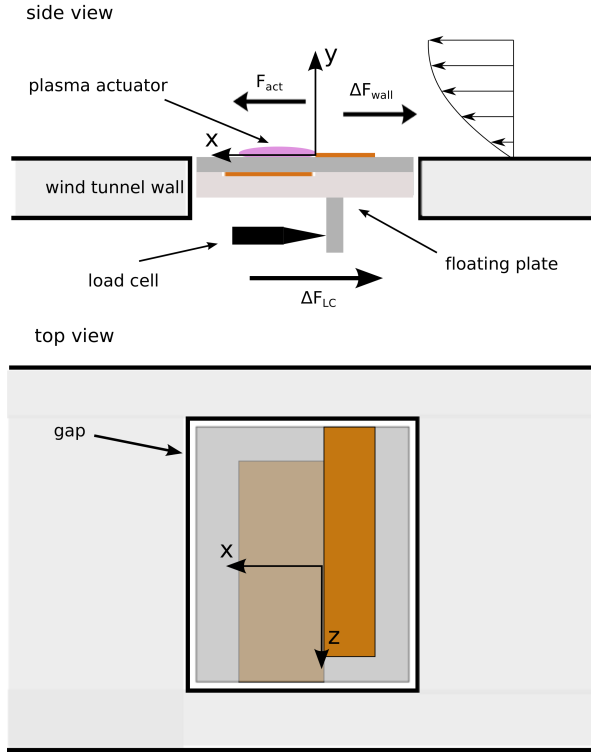
Figure 3.1: Arrangement of the experimental setup (not to scale). Direction of forces corresponds to co-flow forcing configuration.
