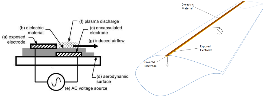
Figure 2.7: Plasma Actuator Diagram - Left DBD Representation - Right Working Schematic of DBD Actuator on HAWT Blade
