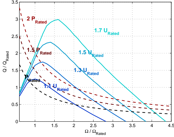
Figure 7.2: NREL rotor loading obtained without blade pitching above rated wind speeds
