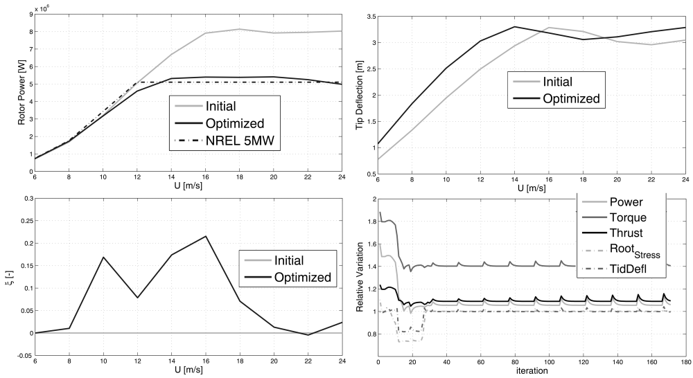
Figure 7.8: Optimization Results - Operational Load Envelope
