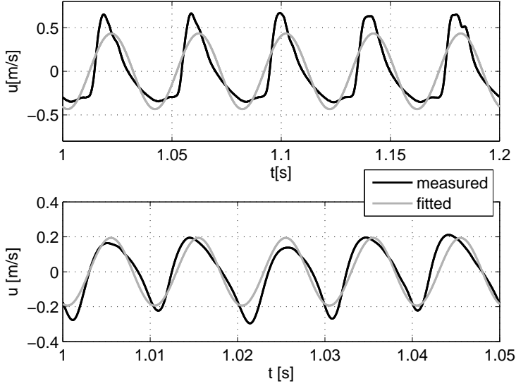
Figure 4.5: Experimental and fitted single harmonic perturbation velocity at quiescent conditions for f_p = 25 Hz (top) and f_p = 100 Hz (bottom)
