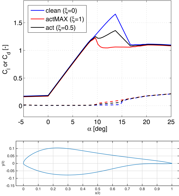
Figure 7.3: WAP 20 – 18C – PD Airfoil top - Aerodynamic Characteristics for clean and actuated MAX operation bottom - Section Contour
