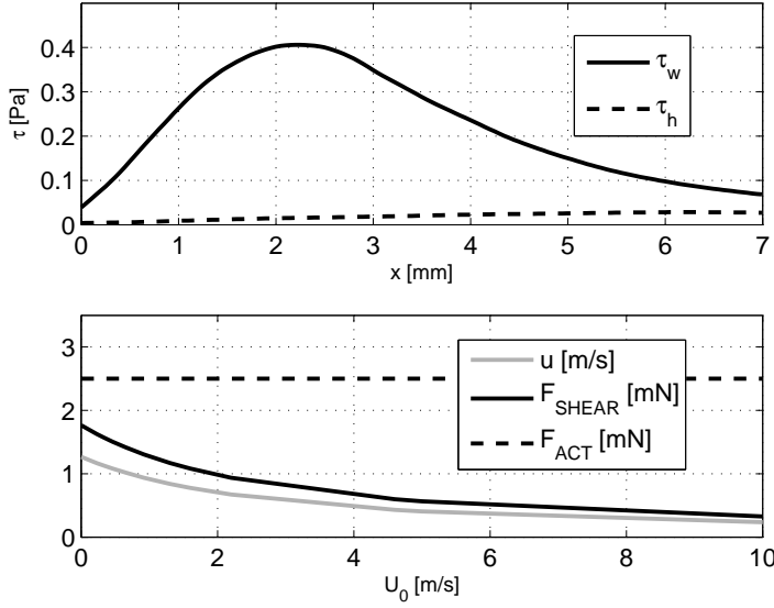
Figure 4.4: top -Experimental shear stress distribution [71] and bottom - modeled perturbation velocity and shear versus external velocity
