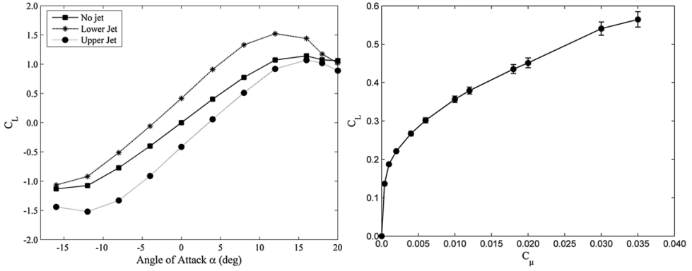
Figure 2.6: C_l of a NACA 0018 airfoil at Re = 6.6 \times 10^5 and Ma = 0.176 with TEJ located at x/c = 0.9 and h_{jet} = 0.006c from [15]. Left- C_l vs \alpha for C_\mu = 0.012 and Right - C_l vs C_\mu for \alpha = 0^\circ
