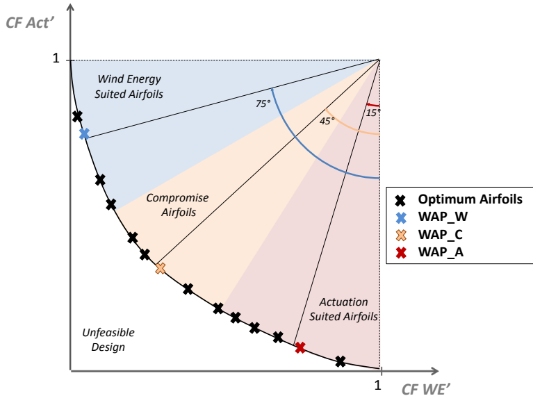
Figure 6.3: Illustration of Compromise Level Selection Procedure
