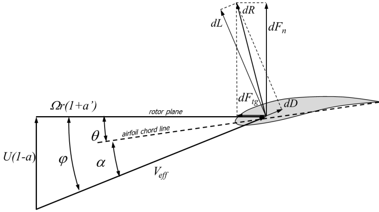
Figure 2.1: Blade Element Decomposition (courtesy of Nando Timmer)
