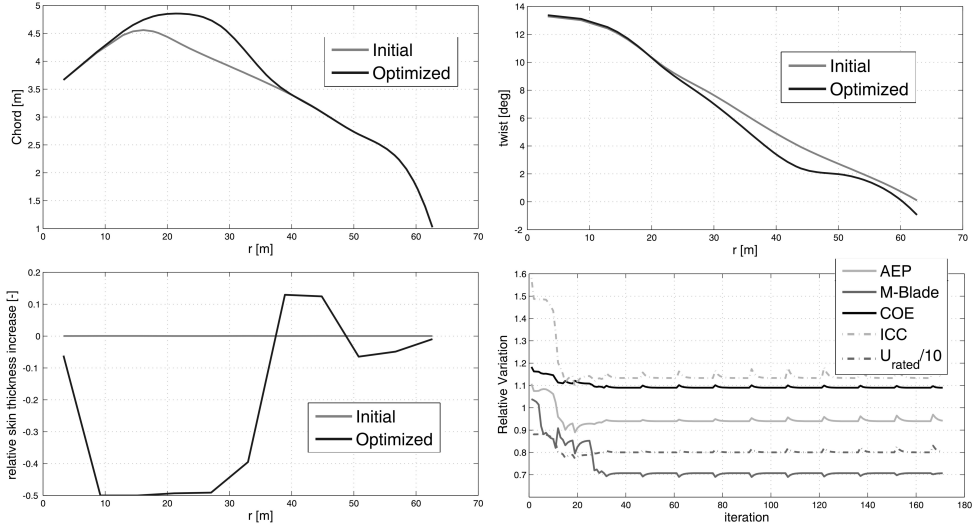
Figure 7.7: Optimization Results - Planform Variables Evolution
