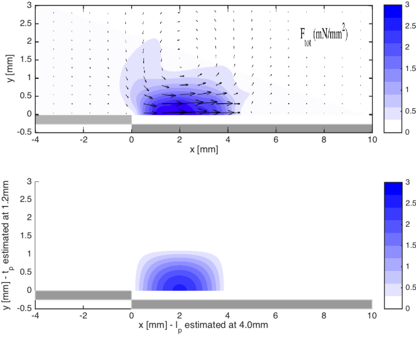
Figure 5.1: top - The force field distribution from reference [69] and bottom - its approximation
