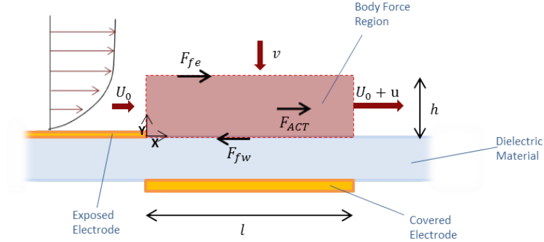
Figure 4.2: DBD Actuator Control Volume (Not to scale)
