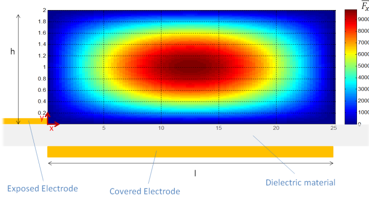
Figure 2.9: Assumed DBD Body Force Spatial Distribution for Turbulent Separation Assessment
