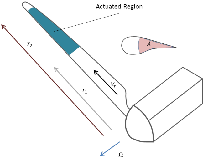
A2 - Sketch defining variables for the Power Consumption
