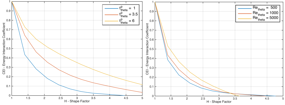
Figure 5.2: Small Perturbation Numerical Estimation of the Energy Interaction Coefficient - left - Influence of t_{\theta}^p and right - Influence of Re_{\theta}
