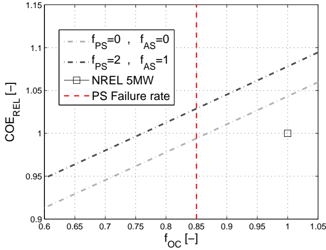
Figure 7.9: Estimated COE versus operation/maintenance f_{OC} cost, under different scenarios of actuation system f_{AS} and pitch system f_{PS} cost. Vertical dashed line indicates failure rate of state-of-the art pitch systems [23]
