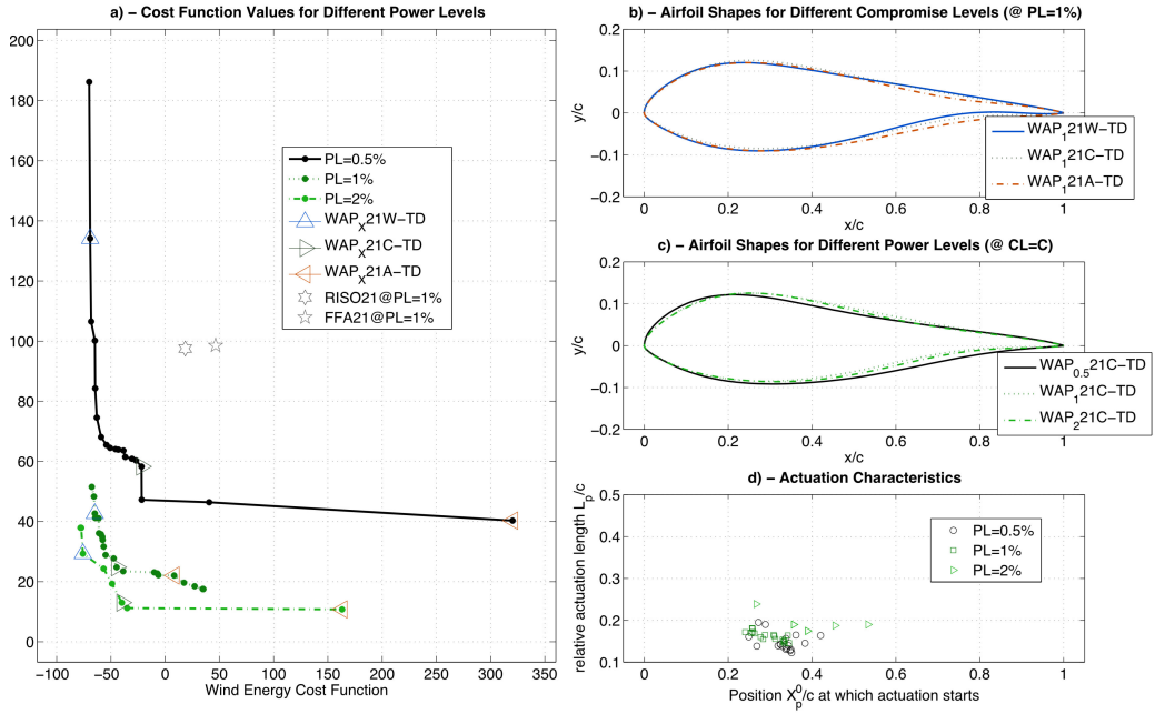
Figure 6.4: WAP - Transpiration Decreased Performance - a) Cost Function Values, b) Compromise Level Shapes, c) Power Level Shapes, d) Actuation Characteristics
