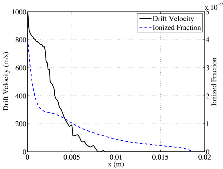
Figure 3.9: Imposed ion drift velocity and ionization fraction spatial distribution
