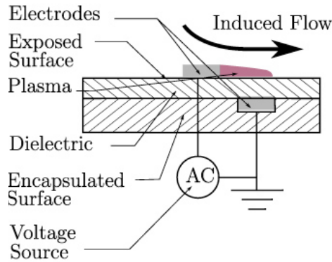
Figure 1.3: Schematic Representation of a DBD Plasma actuator (adapted from [46])
