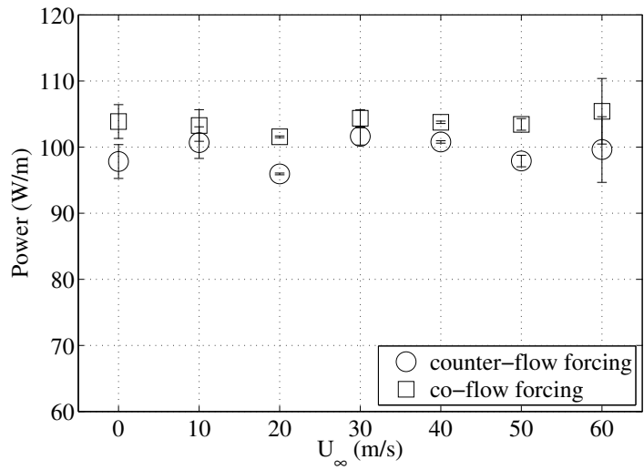
Figure 3.3: Power consumption
