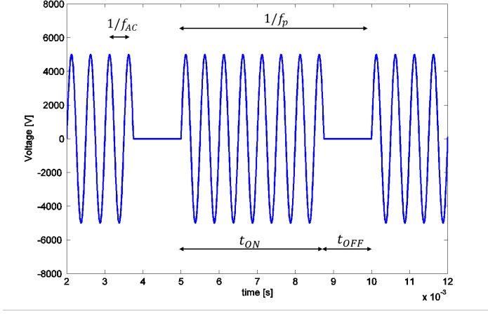
Figure 4.3: Sample of the voltage signal with characteristic actuation values f_{AC} = 2\text{kHz} , f_p = 200\text{Hz} and DC = 75\%
