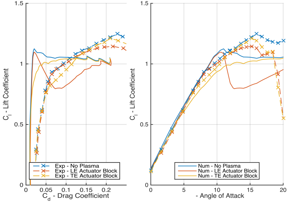
Figure 5.8: C_l and C_d Experimental and Computed Polars at U_\infty = 20 \text{ m/s}
