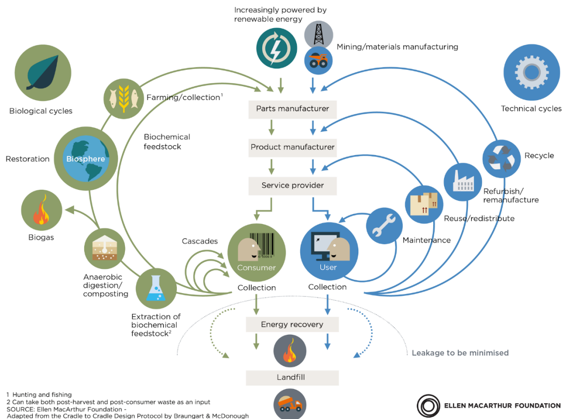
Fig. 1. Butterfly Diagram from the Ellen MacArthur Foundation showing the circular strategies [14].
