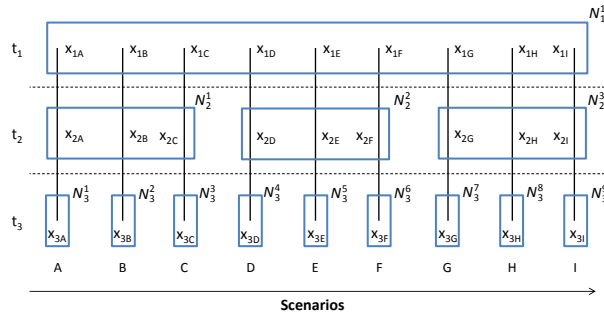
Figure 2: Scenario tree constraints example
