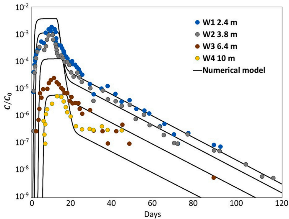
Fig. 5. Comparison of modeled and measured MS2 breakthrough curves of field test experiment (Schijven et al., 1999). The simulation parameters are v_D = 0.5 m/d, \alpha = 0.01 m, \theta = 0.35 , K_{att} = 1.26 /d, K_{det} = 0.0008 /d, \mu_l = 0.03 /d, and \mu_s = 0.09 /d.
