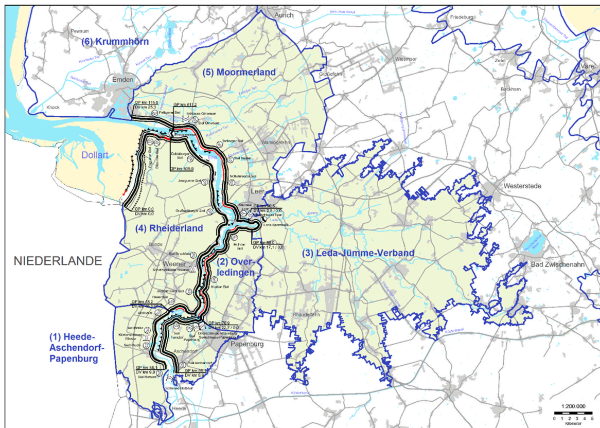
Fig. 3. Deichverband (DVB) along the Ems-Dollard estuary: Heede-Aschendorf-Papenburg (1), Overledingen (2), Leda-Jümme-Verband (3), Rheide (4), Moormerland (5) and Krümmhörn (6) (green-line). Thick-black-line: Heightened Dyke, thick-red-line: under construction dyke, thin-black-line: available dyke protection roads, thin-red-line: required dyke protection road, black-saw-line: revetment area (NLWKN, 2007). (For interpretation of the references to colour in this figure legend, the reader is referred to the Web version of this article.)
