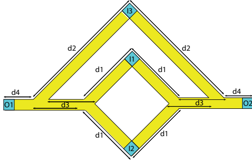
Fig. 3. Fan-out of 2 MAJ3 Gate.
