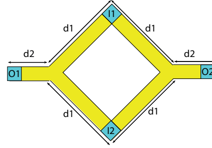
Fig. 4. Fan-out of 2 XOR Gate.
