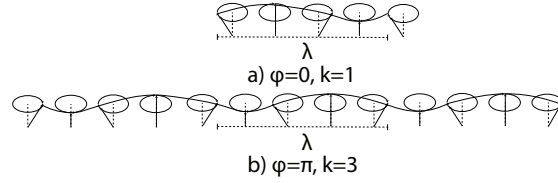
Fig. 1. Spin Wave Parameters.
