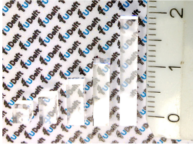
Figure 4. Photograph of the BGO samples tested in this work. All crystals have a cross-section of 3\text{ mm} \times 3\text{ mm} . From left to right, the crystal lengths are 3 mm, 5 mm, 8 mm, 12 mm, and 20 mm.
