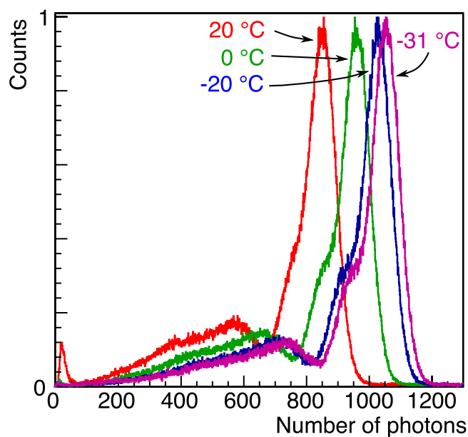
Figure 6. Normalized energy spectra of one of the two 3 mm \times 3 mm \times 3 mm BGO detectors measured in coincidence at 4 different temperatures.
