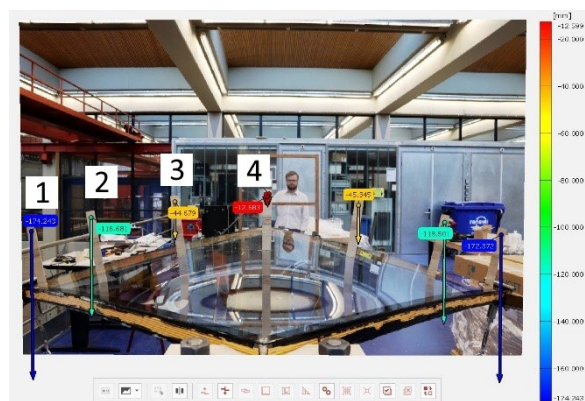
Fig. 12: 2D displacements at specific points measured with 2D DIC. Displacements in vertical direction are displayed. The numbering system for the points is also shown (points 1-4).
