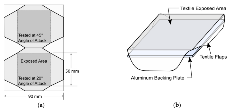
Figure A1. Preparation of fabrics for the flat plate configuration. (a) The exposed portion of fabric tested with respect to its original size; (b) Placement of the fabric on a rigid backing plate indicating the folding style of the flaps.
