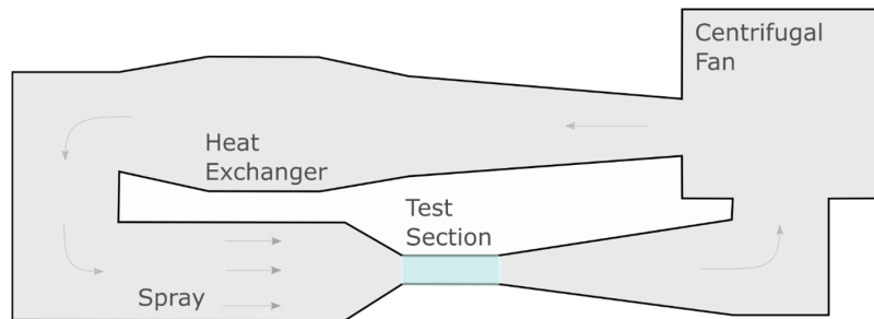
Figure 2. Icing wind tunnel.
