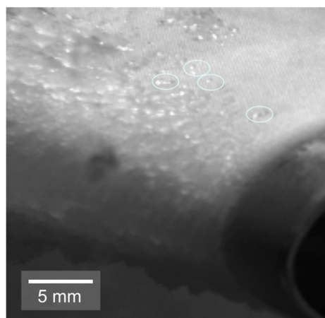
Figure A3. Ice formation on the fabric mounted on a NACA 0012 airfoil showing isolated feathery ice grains near the top side (circled) that become more dense and homogenous approaching the stagnation line.
