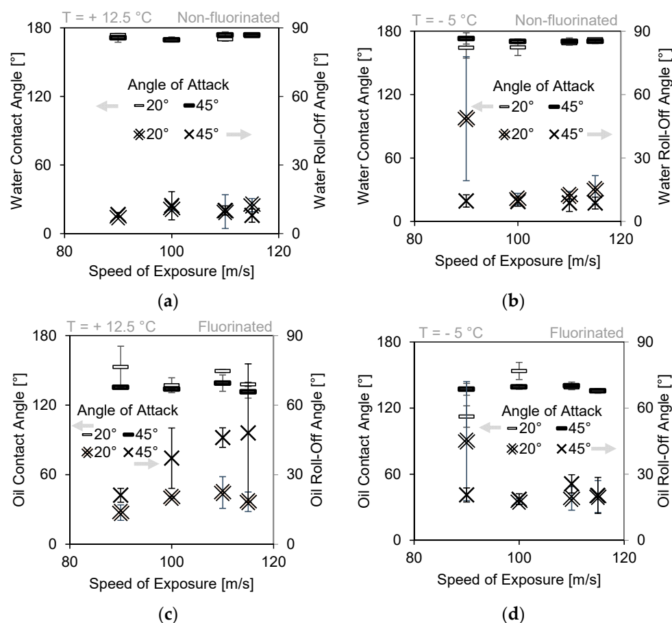
Figure 6. Wetting properties of fabrics exposed to cloud conditions for 10 min at increasing speeds while on a flat plate at an angle of attack of 20° (horizontal dash) and 45° (cross). (a) Water droplets on a superhydrophobic fabric after exposure at +12.5 °C. (b) Water droplets on a superhydrophobic fabric after exposure at −5 °C. (c) Oil droplets on a superamphiphobic fabric after exposure at +12.5 °C. (d) Oil droplets on a superamphiphobic fabric after exposure at −5 °C.
