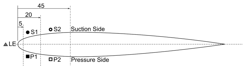
Figure 3. Diagram of the NACA 0012 support with 180 mm-chord length and labels for positions on the fabrics. LE: leading edge, or stagnation line; S1, S2: suction side; P1, P2: pressure side.
