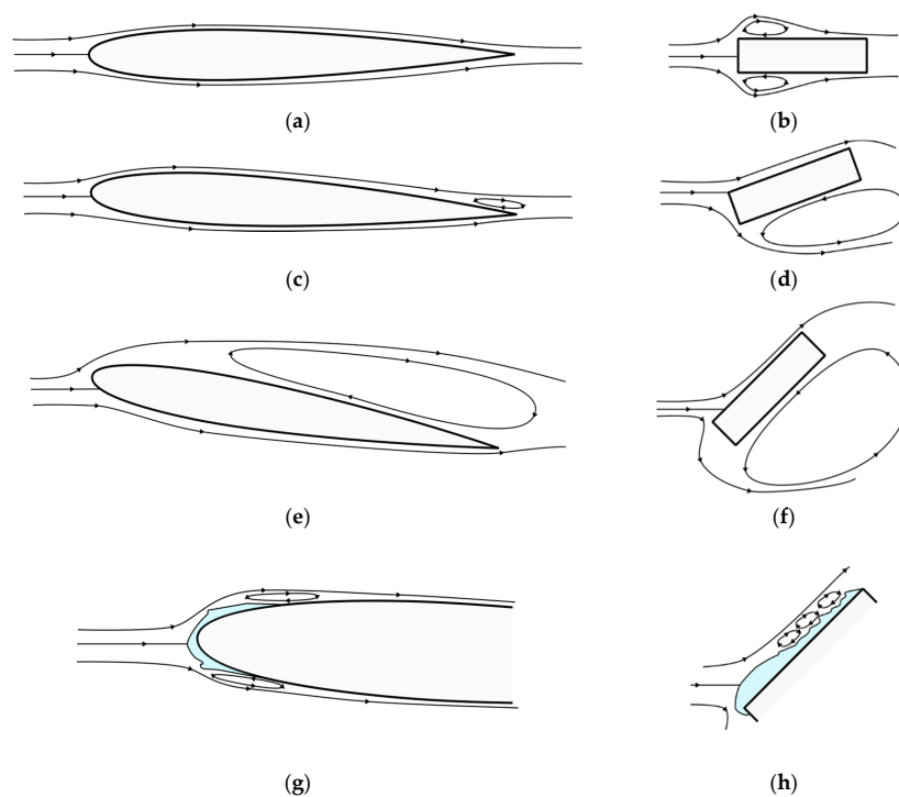
Figure A2. Pathlines over NACA 0012 and flat-plate sample holders at various angles of attack and with an arbitrarily low Reynolds Number. (a) Airfoil at 0^\circ angle of attack (AoA) showing symmetric pathlines without flow separation; (b) Block holder at 0^\circ AoA showing symmetric pathlines with flow separation and reattachment; (c) Airfoil at 3^\circ AoA showing slightly asymmetric pathlines and flow separation at the trailing edge on the suction side; (d) Block holder at 20^\circ AoA showing stagnation at the leading corner, and attached flow along the top side; (e) Airfoil at 10^\circ AoA showing asymmetric pathlines and flow separation along the entire suction side; (f) Block holder at 45^\circ AoA showing an elevated stagnation point and attached flow on the top side; (g) Iced airfoil at 3^\circ AoA showing slightly asymmetric pathlines with small flow separations immediately downstream of the ice; (h) Iced block holder at 45^\circ AoA showing uneven ice with complete coverage of the top side and a series of small flow detachments due to the ice shape; (a, c, e, and g) are based on [31]. (b, d, and f) are reproduced from [26].
