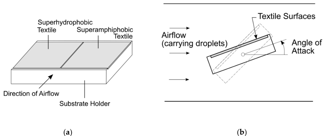
Figure 4. Configuration of fabric mounted to a flat plate sample holder in the icing wind tunnel test section. (a) Side-by-side arrangement of fabrics in the flat plate substrate holder; (b) Side view of the configuration in the test section showing the direction of airflow, top and bottom test section walls, and the two tested angles of the sample holder.
