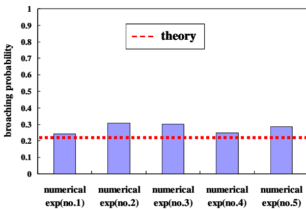
Figure 4 Comparison in broaching probability between numerical experiments and theory for a high-speed fishing craft in irregular stern quartering waves (Umeda et al., 2007).
