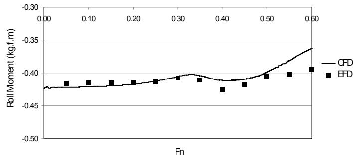
Figure 2 Comparison between the physical model experiment (EFD) and the RANS solution (CFD) in roll moment acting on the ONR tumblehome model running in still water with the heel angle of 10 degrees (Hashimoto and Stern, 2007).
