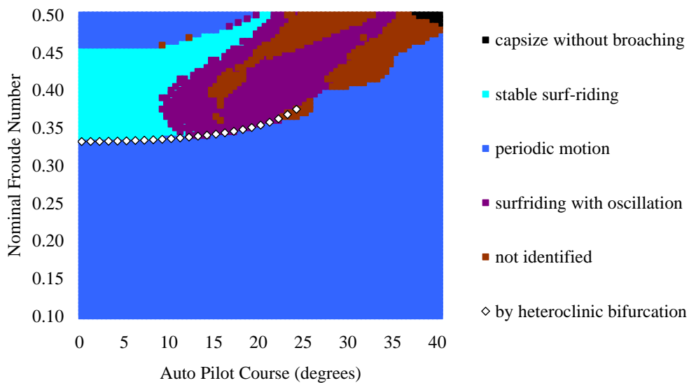
Figure 3 Comparison in motions of the ITTC Ship A-2 running in following waves between numerical simulation results and the heteroclinic bifurcation (Umeda et al., 2006A).
