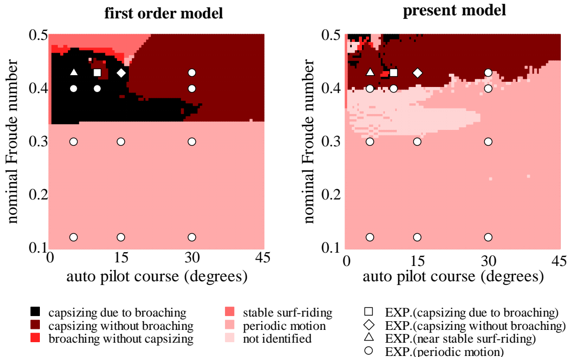
Figure 1 Comparison between the experimental results and numerical results (first order model and present model) for the ITTC Ship A-2 with wave steepness of 0.1 and wavelength to ship length ratio of 1.637 (Umeda and Hashimoto, 2006C).
