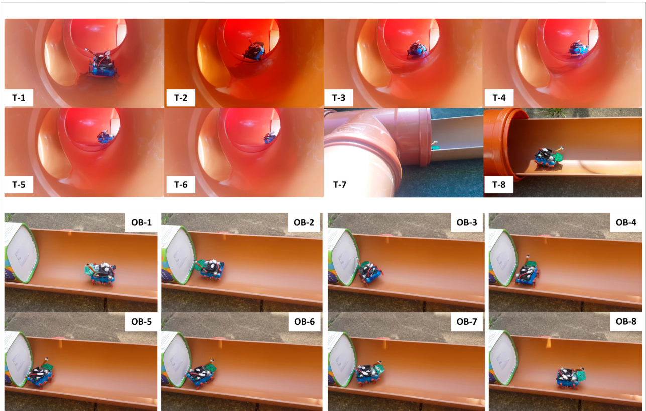
FIGURE 9 Successful detection, decision making and maneuvers of the Joey robot at T-junction (T-1 to T-8, top two rows) and large obstacle (OB-1 to OB-8, bottom two rows) in autonomous pipe exploration.
