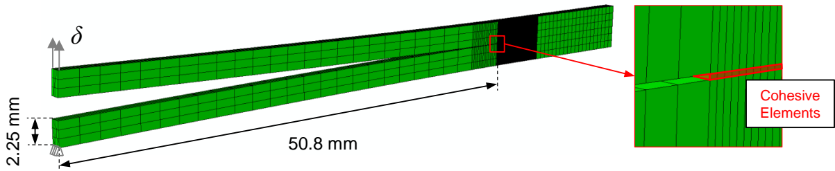
Figure 4: DCB FE model.
